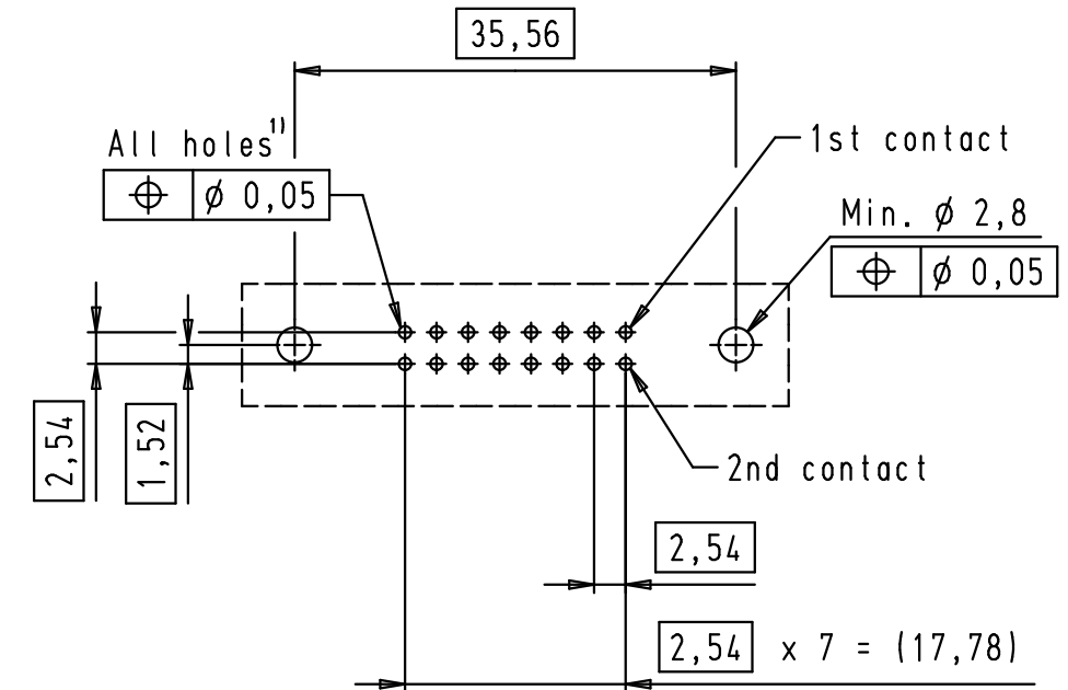
PCB layout, component side
