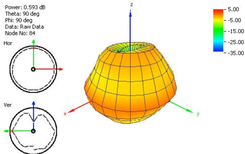
Figure 10. Radiation Pattern at 2460 MHz.
