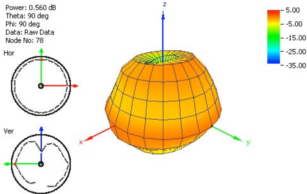
Figure 11. Radiation Pattern at 2460 MHz.
