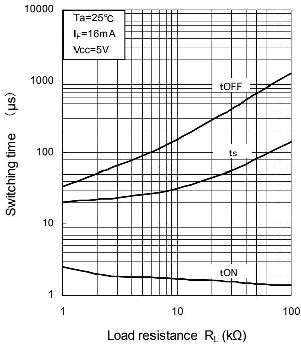
Switchingtime — R_L
