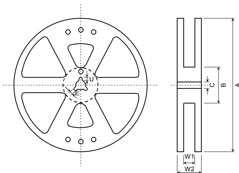
Figure 3 Reel Forms
