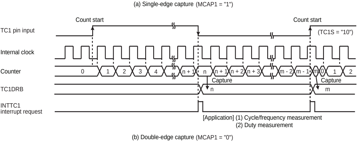
Figure 8-6 Pulse Width Measurement Mode
