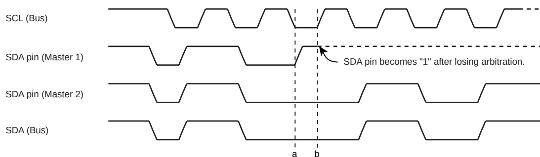
Figure 16-7 Arbitration Lost
