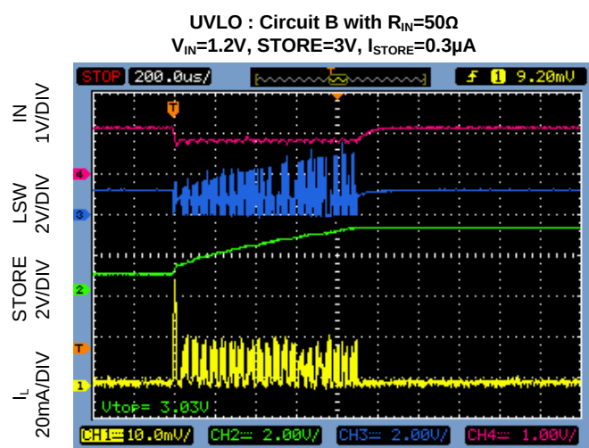
Figure 1. TS3310, UVLO=0.855V
