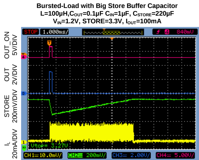
Figure 7. 220µF C_{STORE} Recovery Scope Capture
