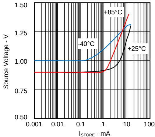
Minimum Start-Up Voltage vs STORE Output Current Circuit A with 10 \Omega Source Resistance (STORE=1.8V)
