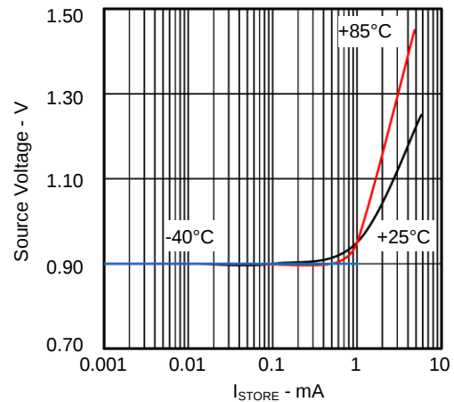
Minimum Start-Up Voltage vs STORE Output Current Circuit B with 10 \Omega Source Resistance (STORE=3V)
