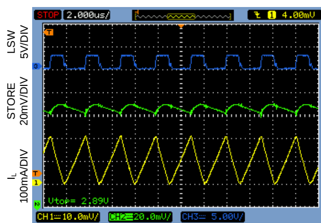
STORE Output Voltage Ripple, Inductor Current, and LSW Voltage : Circuit A V_{IN}=1.2V , STORE=3V , I_{STORE(MAX)}=35mA
