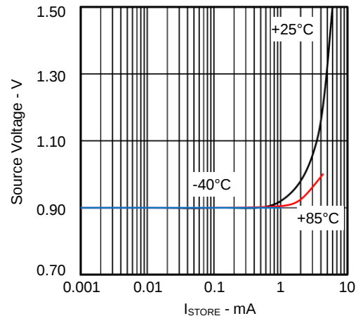
Minimum Start-Up Voltage vs STORE Output Current Circuit B with 10 \Omega Source Resistance (STORE=1.8V)
