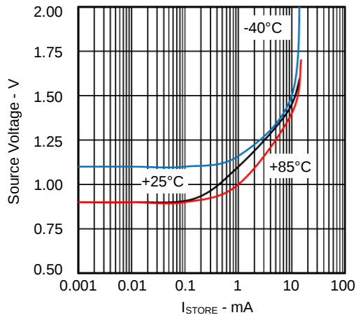
Minimum Start-Up Voltage vs STORE Output Current Circuit A with 10 \Omega Source Resistance (STORE=3V)
