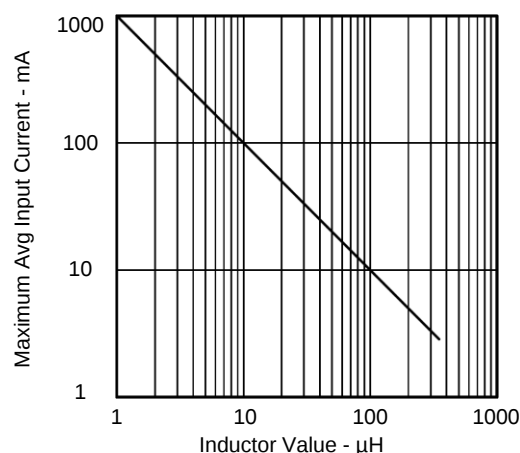
Figure 3. I_{IN(AVG,MAX)} vs Inductor Value
