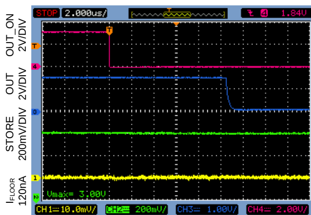
OUT_ON Switched OFF : Circuit A with C_{OUT} Removed V_{IN}=1.2V , STORE=3V , I_{STORE}=0.3\mu A , I_{OUT}=3mA
