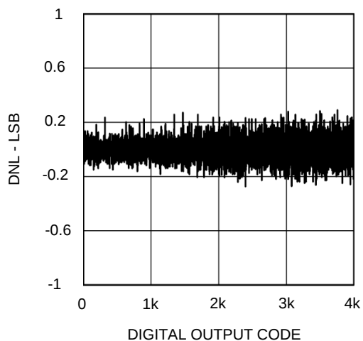
Differential Nonlinearity
