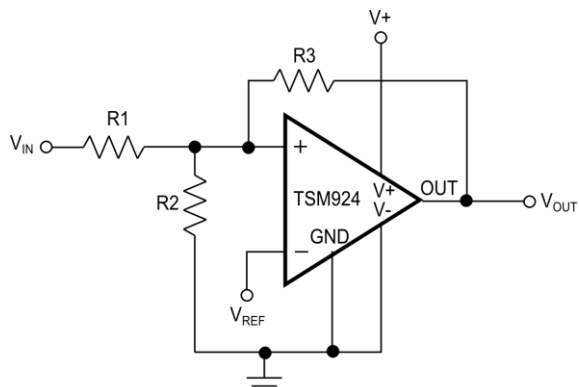
Figure 3. External Hysteresis
