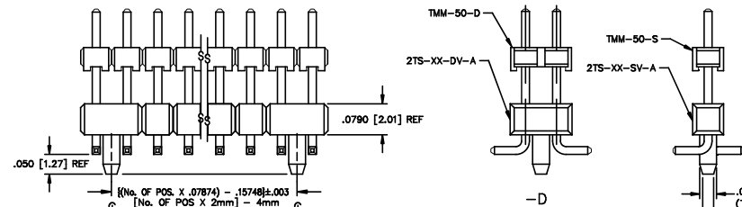
FIG. 3 (-A MOLDED ALIGNMENT PIN OPTION) SAME AS FIG 1 EXCEPT WHERE NOTED. (* = SEE NOTE 12)
