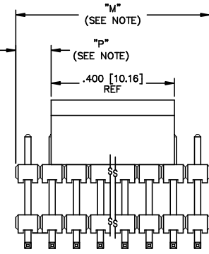
FIG. 5 (-M OPTION) (SEE NOTE 10)
