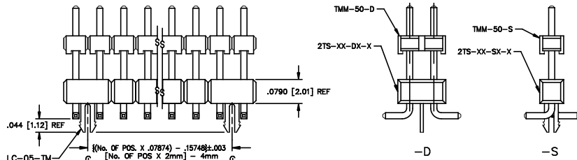
FIG. 2 (-LC OPTION) SAME AS FIG 1 EXCEPT WHERE NOTED.
