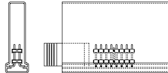
PAGING VIEW SCALE: .5X PT-1-24-02-47 TP-03 ORIENT PLUG SQUARE AT BOTTOM OF TUBE, PINS CANNOT CONTACT THE PLUG.
