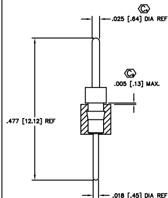
FIG. 2 TERMINAL STYLE -A T-1R0-X
