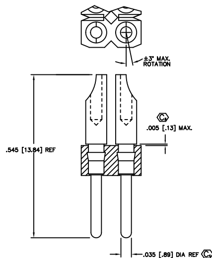
FIG. 7 TERMINAL STYLE -B-2 T-1R8-2-X
