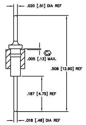
FIG. 19 TERMINAL STYLE -G-1 T-1R5-1-X
