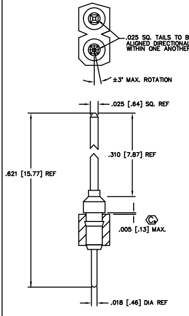
FIG. 12 TERMINAL STYLE -D-1-2 T-1S4-1-2-X
