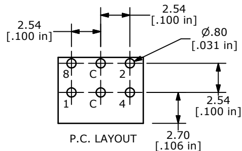
COMPLEMENT CODE
