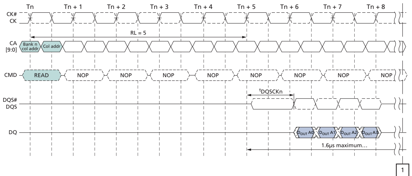
Figure 18: t_{DQSKDM} Timing
