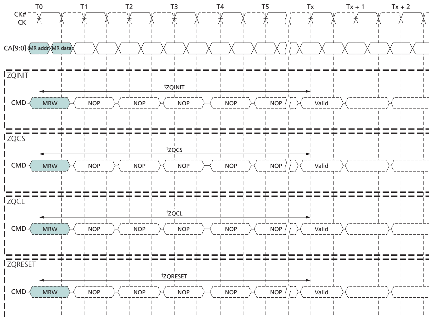
Figure 51: ZQ Timings
