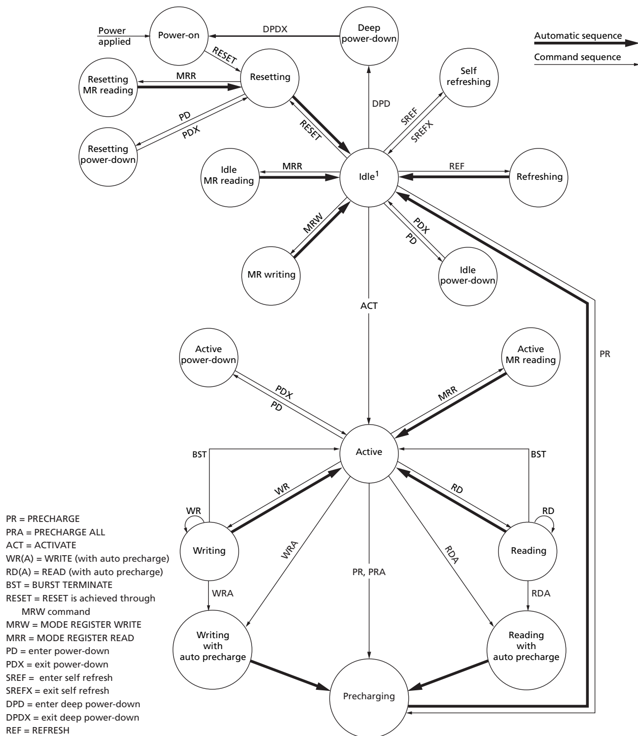
Figure 65: Simplified Bus Interface State Diagram
