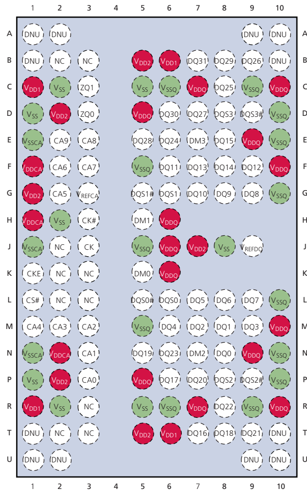
Figure 8: 134-Ball DDP FBGA (x32) Ball Assignments (Top View, Balls Down)
