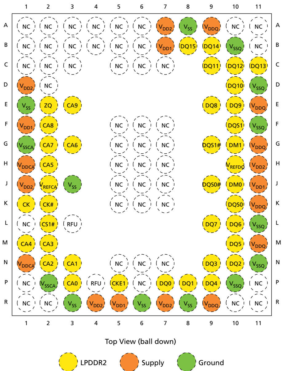
Figure 7: 121-Ball FBGA (x16) Ball Assignments
