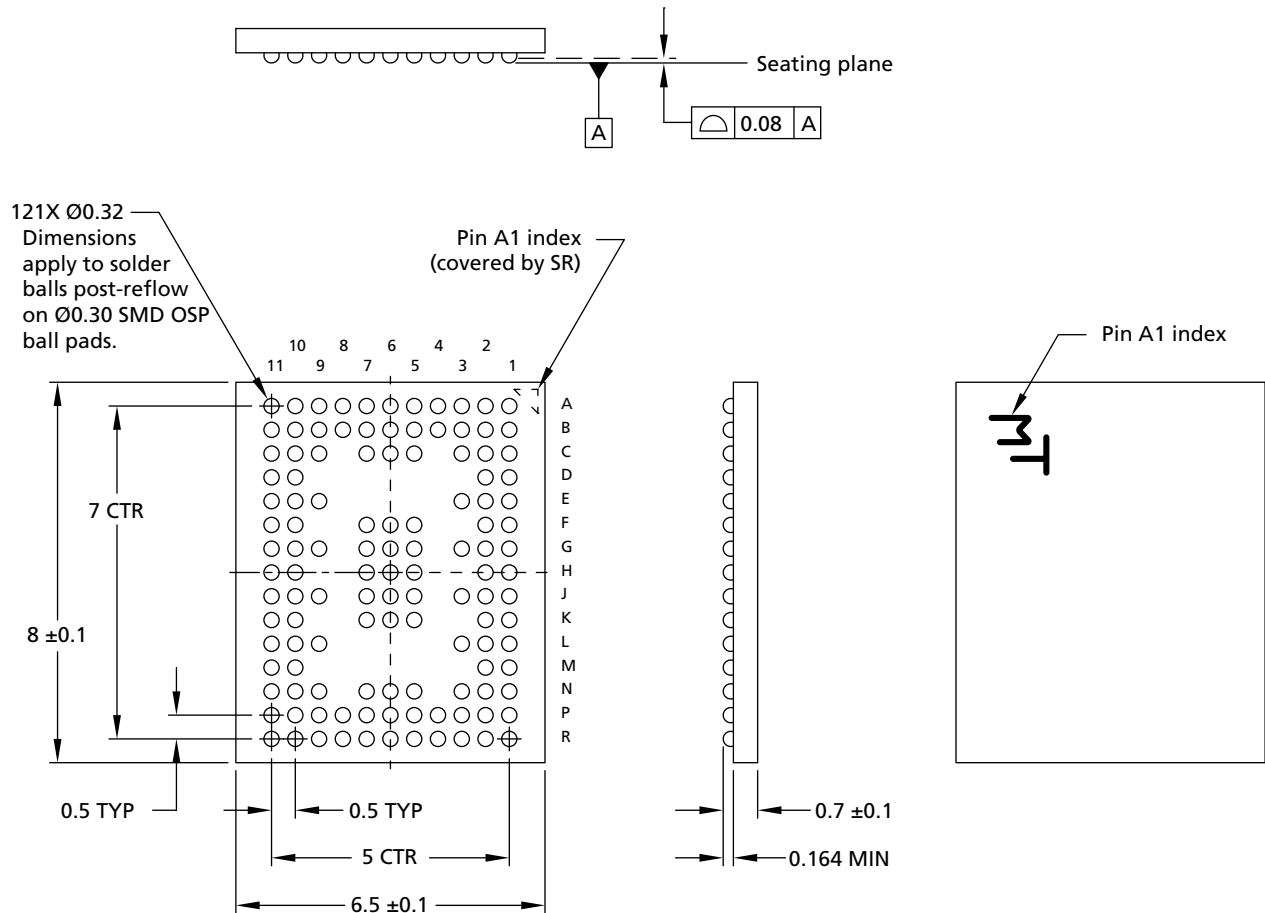
Figure 5: 121-Ball FBGA – 6.5mm x 8mm (Package Code AB)
