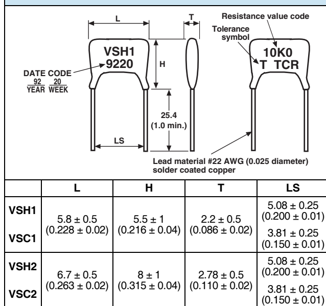
FIGURE 1 - STANDARD IMPRINTING AND DIMENSIONS in millimeters
