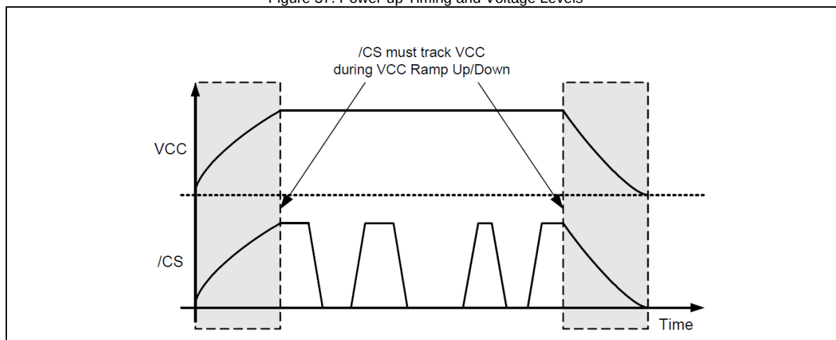
Figure 37b. Power-up, Power-Down Requirement
