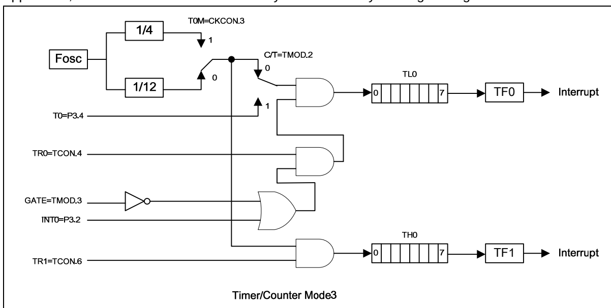
Figure 11-3 Timer/Counter 0 Mode 3
