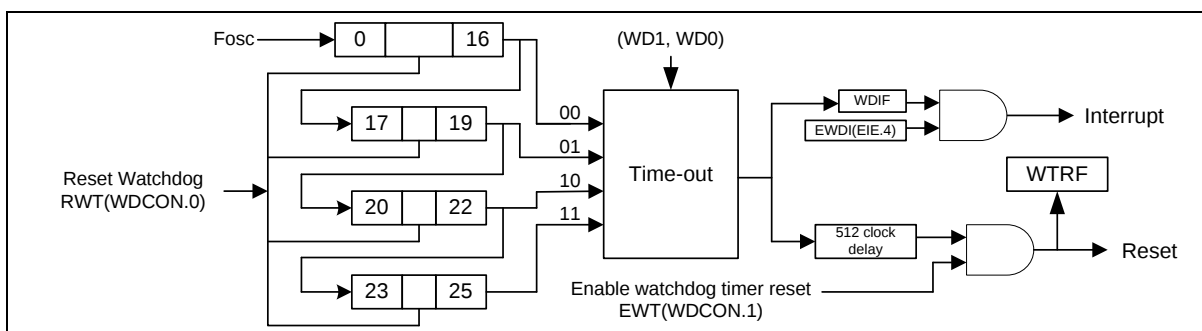
Figure 12-1 Watchdog Timer
