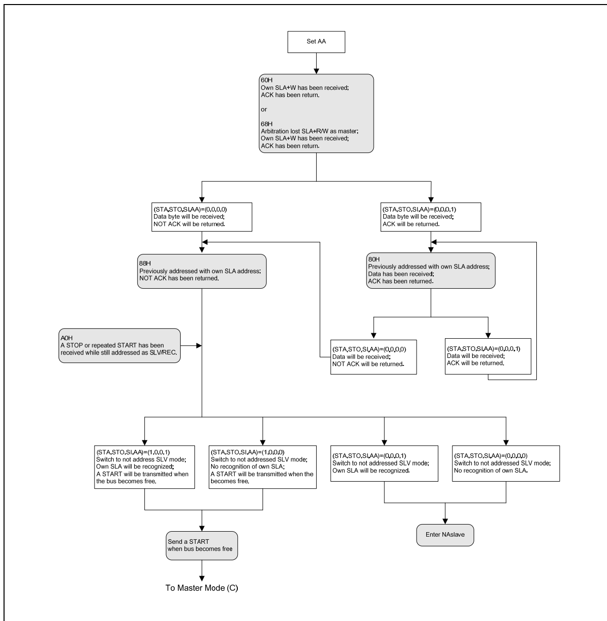
Figure 15-8 Slave Receiver Mode
