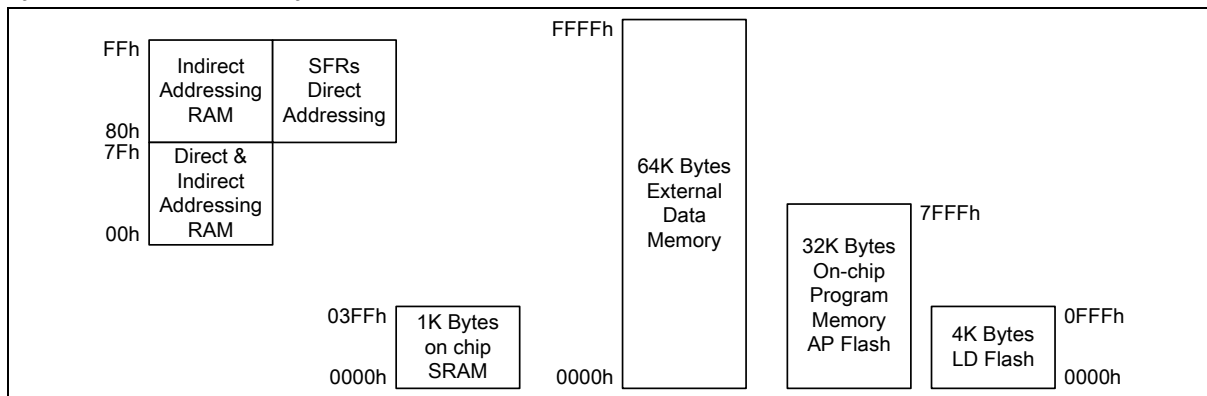
Figure 5-1 Memory Map
