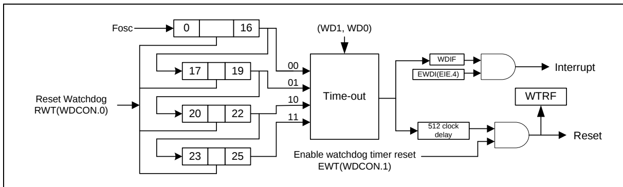
Figure 12-1 Watchdog Timer
