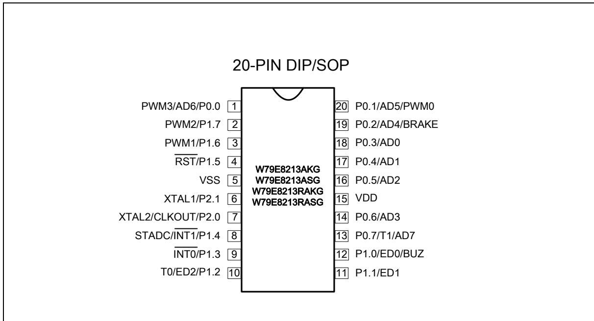
Figure 4-1: Pin Configuration
