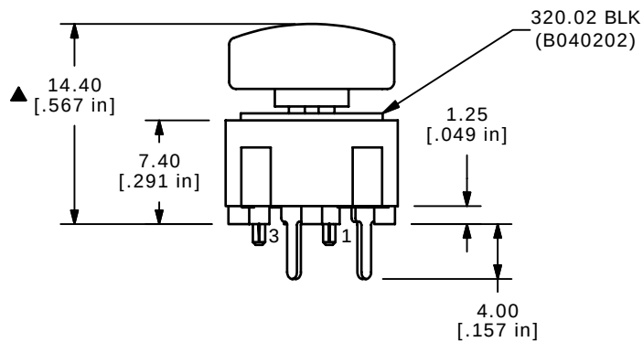
CIRCUIT: SPST CONTACT CONFIGURATION
