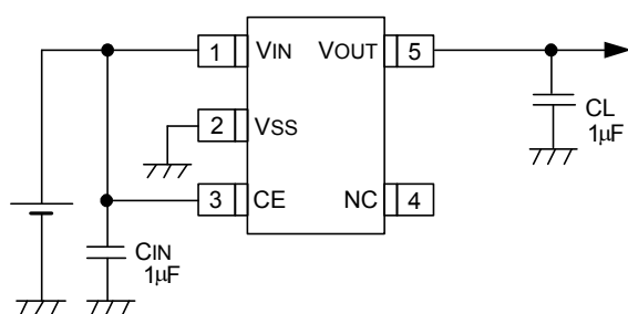
SOT-25 (SOT-23-5)
