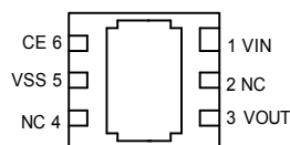
USP-6B (BOTTOM VIEW)
