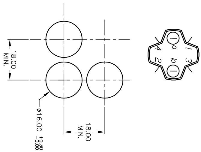
RECOMMENDED PANEL MOUNTING SCALE 1:1
