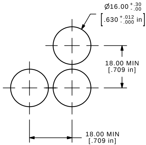
PANEL MOUNTING
