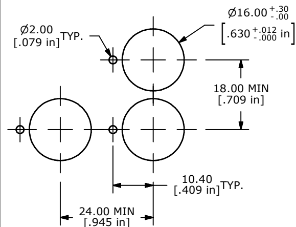
PANEL MOUNTING
