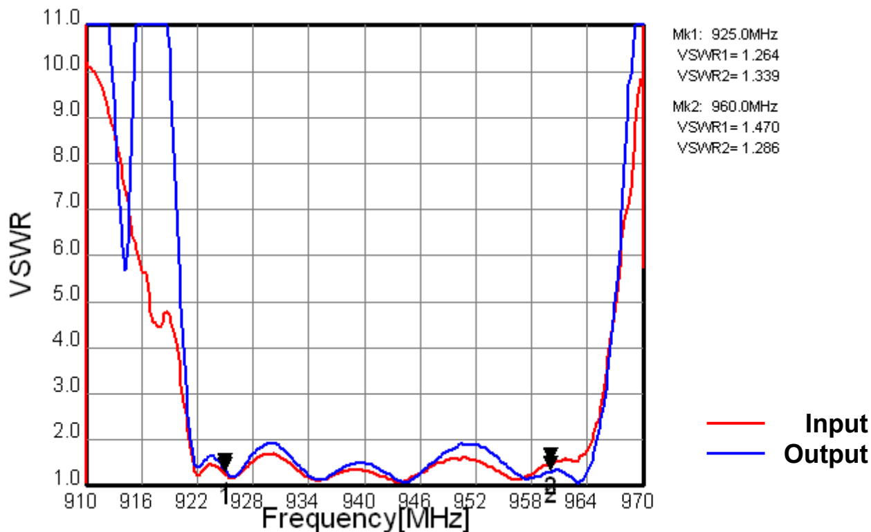
Fig.2 VSWR (Filter1)
