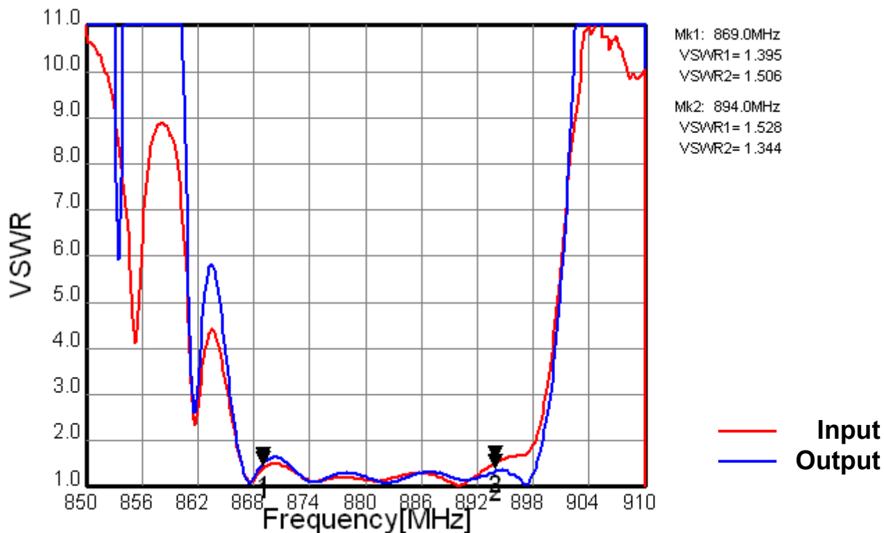
Fig.10 VSWR (Filter2)
