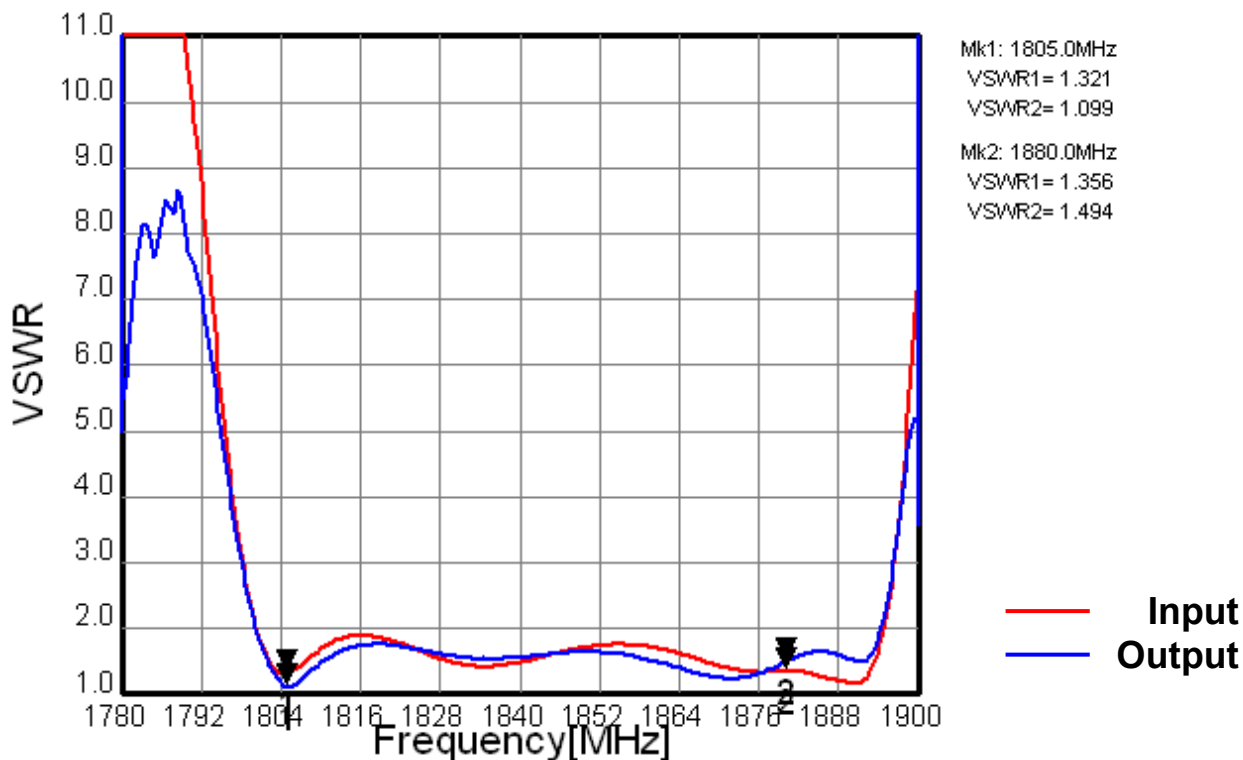
Fig.2 VSWR (Filter1)
