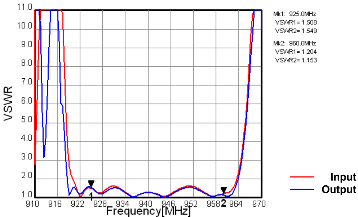
Fig.10 VSWR (Filter2)
