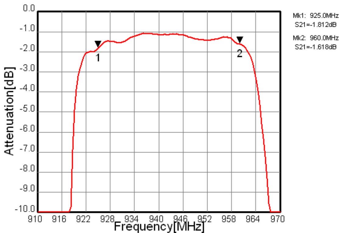
Fig.11 In-band Characteristic (Filter2)
