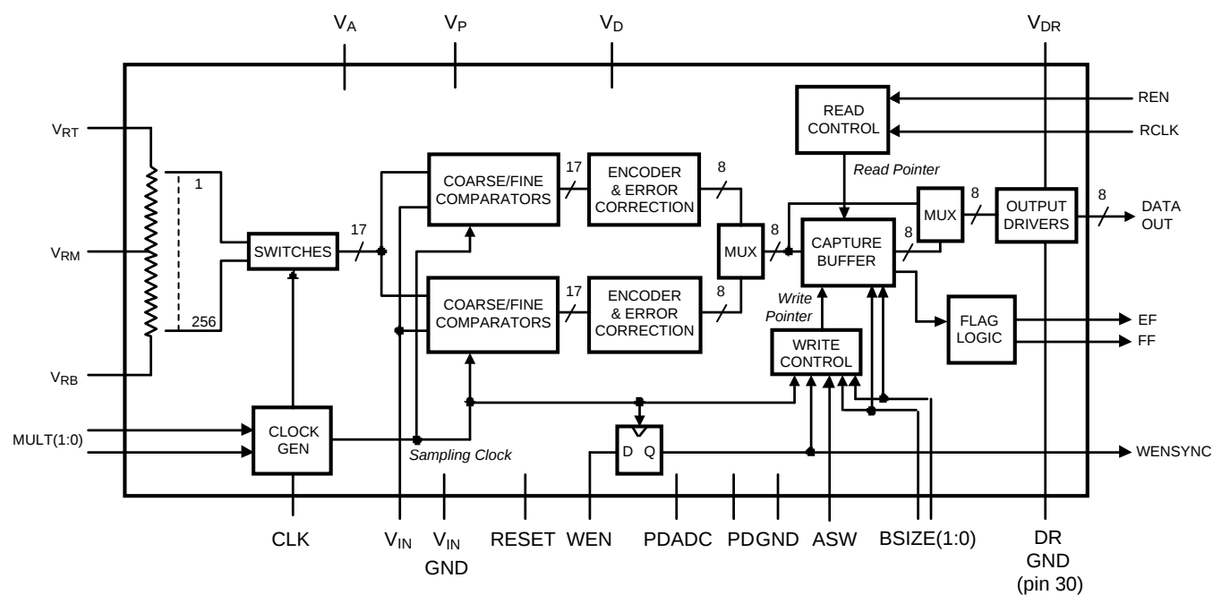
Block Diagram
