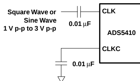
Figure 26. AC-Coupled Single-Ended Clock Input
