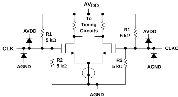
Figure 20. Clock Inputs
