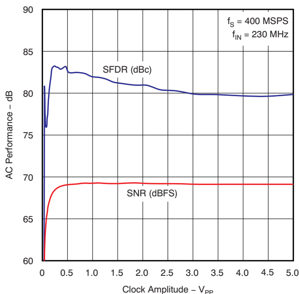
Figure 42. AC Performance versus Clock Level
