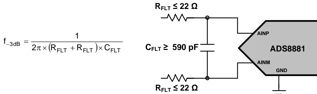
Figure 66. Antialiasing Filter
