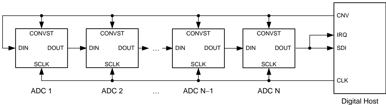
Figure 61. Connection Diagram: Daisy-Chain Mode With a Busy Indicator (DIN = 0)
