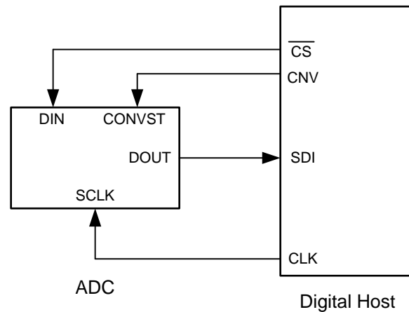
Figure 53. Connection Diagram: Single ADC with 4-Wire \overline{\text{CS}} Mode Without a Busy Indicator
