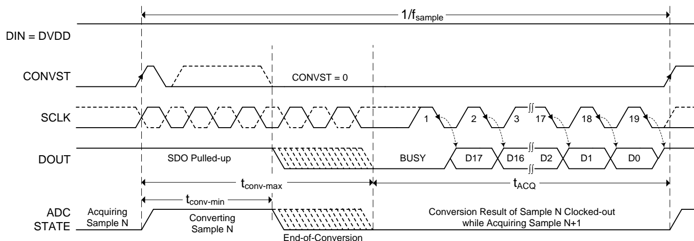
Figure 52. Interface Timing Diagram: 3-Wire \overline{\text{CS}} Mode With a Busy Indicator (DIN = 1)
