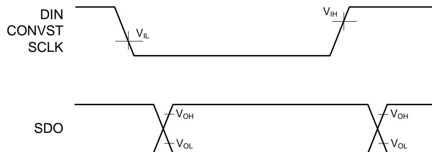
Figure 5. Voltage Levels for Timing
