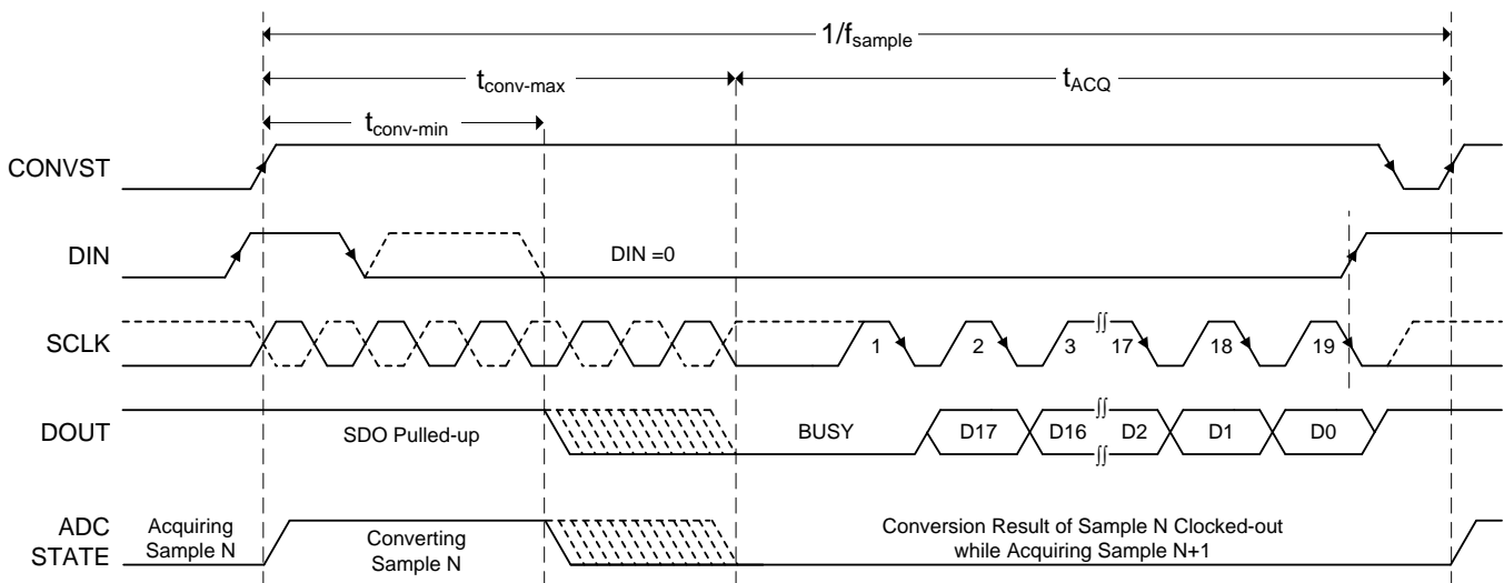
Figure 58. Interface Timing Diagram: 4-Wire \overline{\text{CS}} Mode With a Busy Indicator
