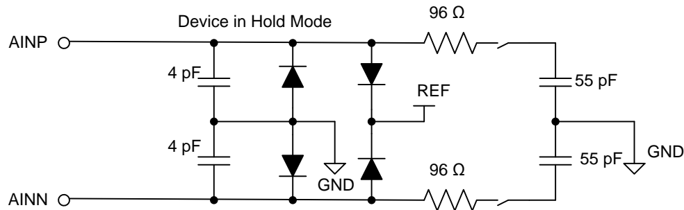
Figure 46. Input Sampling Stage Equivalent Circuit
