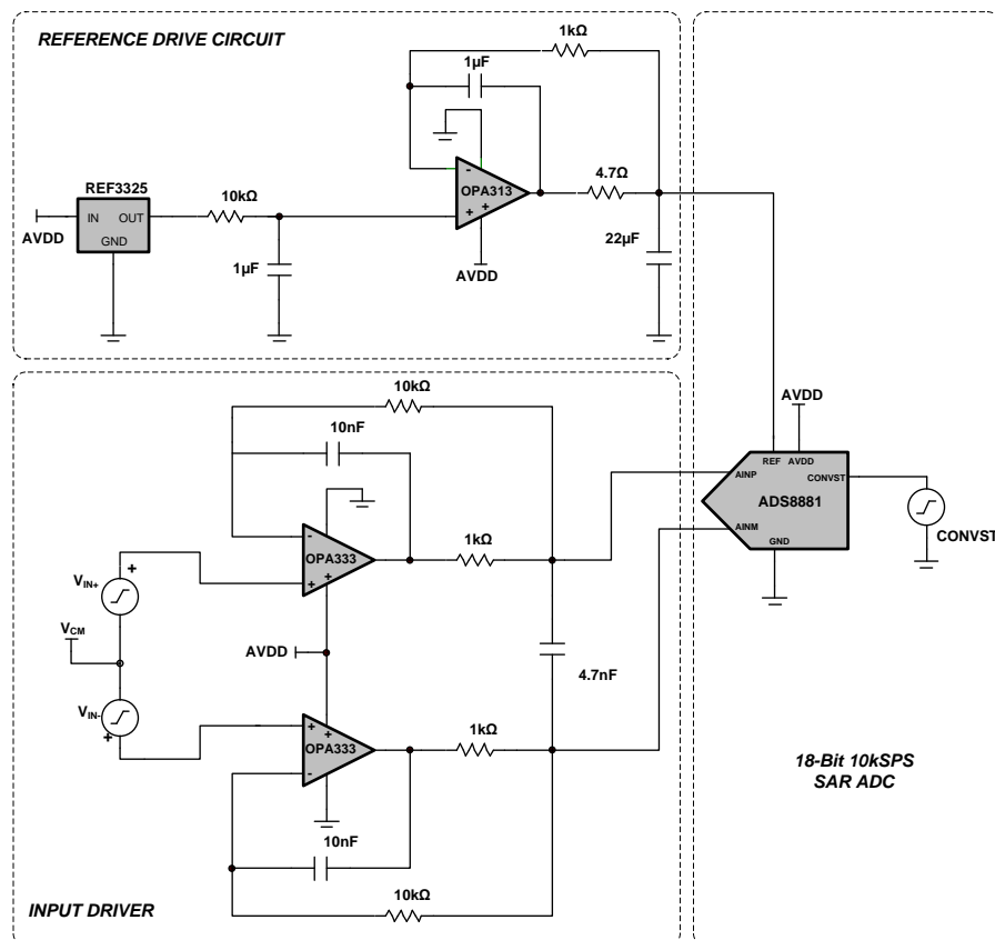
Figure 71. Ultralow-Power DAQ Circuit at 10 kSPS
