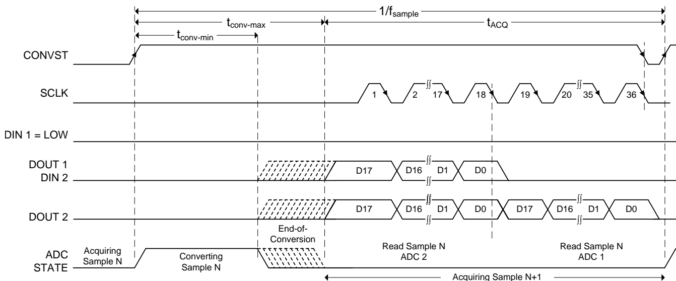
Figure 60. Interface Timing Diagram: For Two devices in Daisy-Chain Mode Without a Busy Indicator
