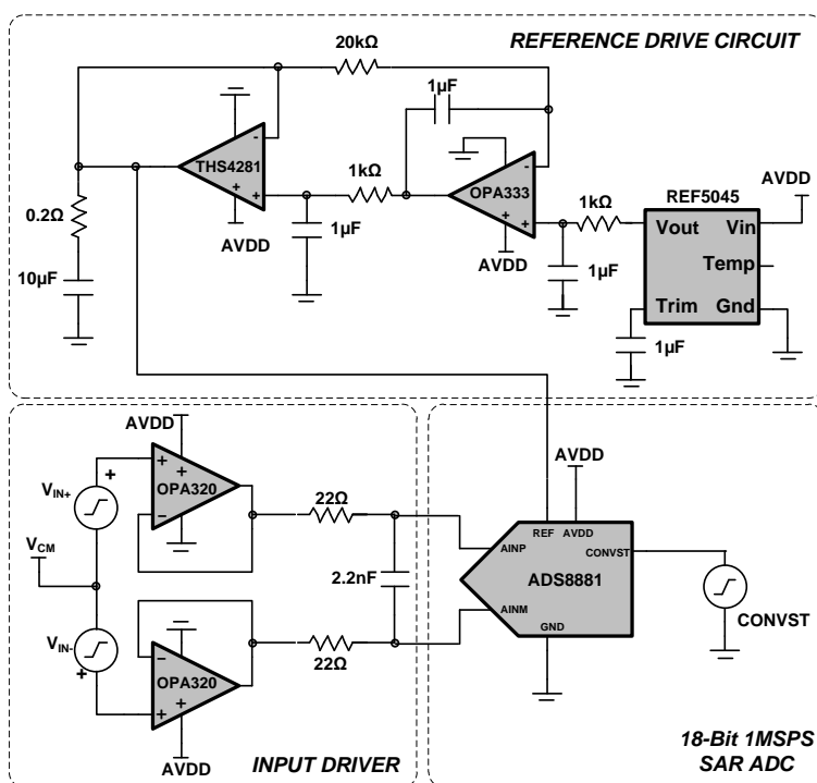
Figure 68. DAQ Circuit for Lowest Power and Excellent Dynamic Performance at 1 MSPS
