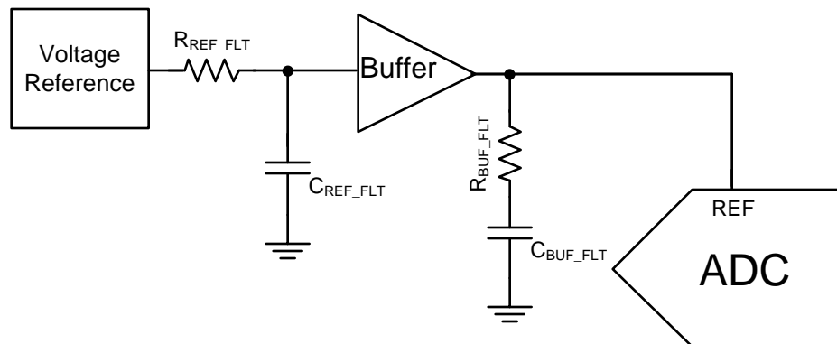
Figure 47. Reference Driver Schematic
