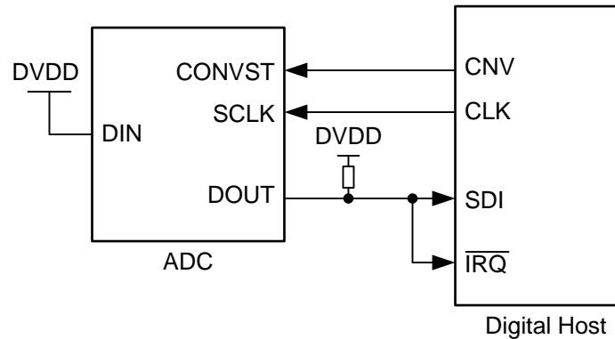
Figure 51. Connection Diagram: 3-Wire \overline{\text{CS}} Mode With a Busy Indicator
