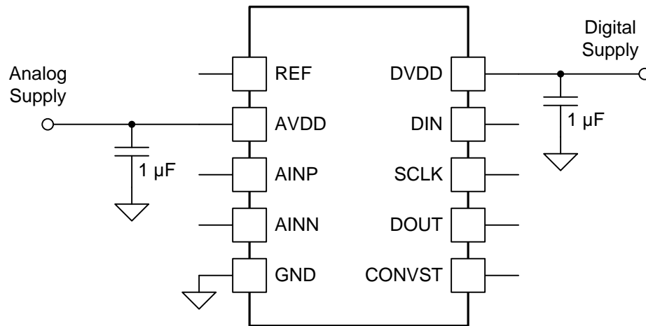
Figure 63. Supply Decoupling
