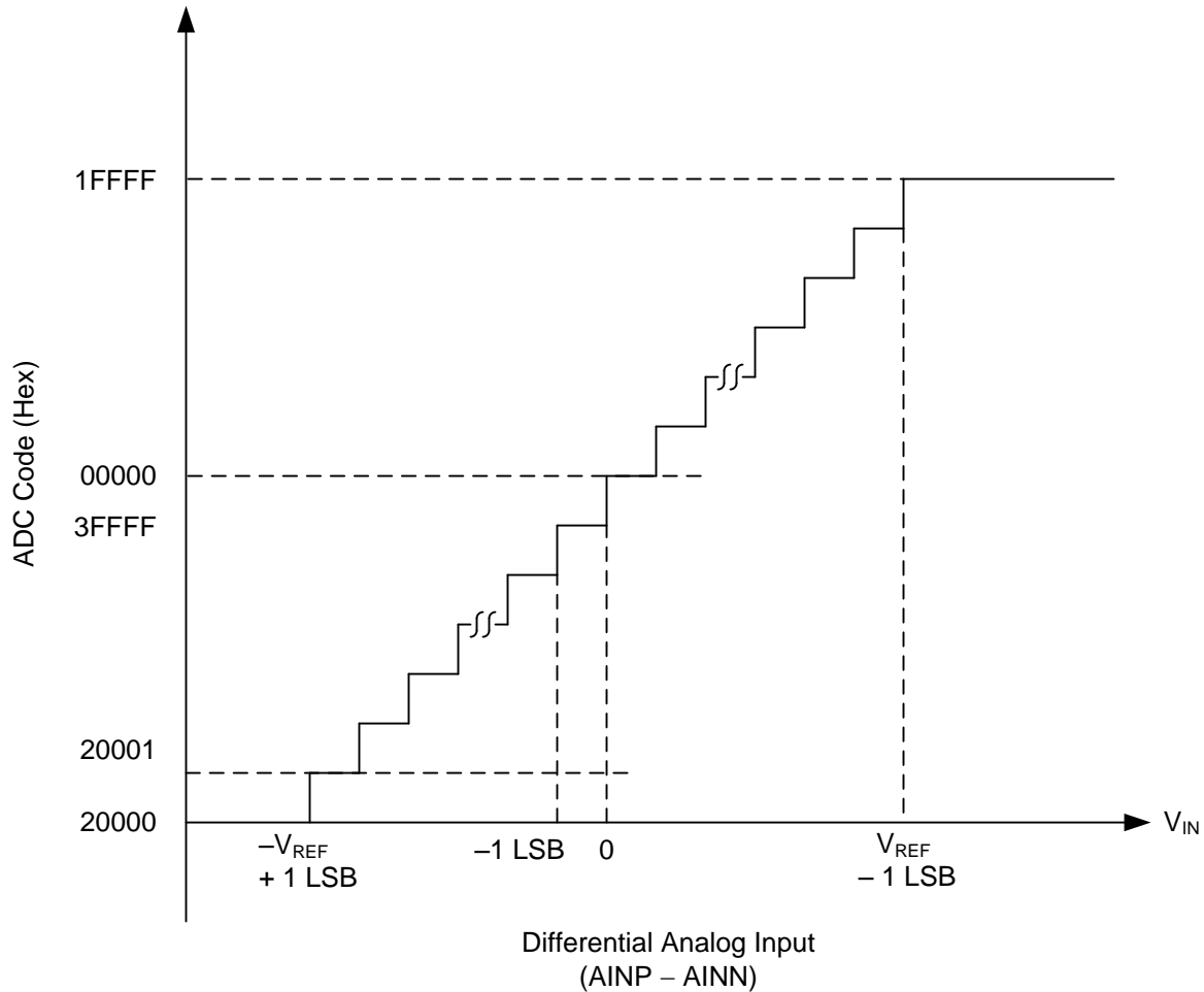
Figure 48. Differential Transfer Characteristics
