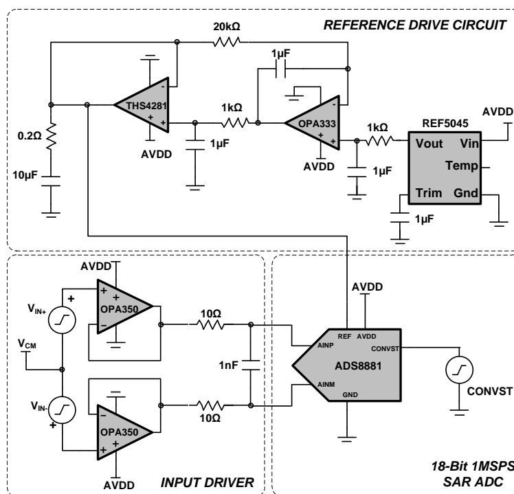
Figure 67. DAQ Circuit for 1- \mu s, Full-Scale Step Response
