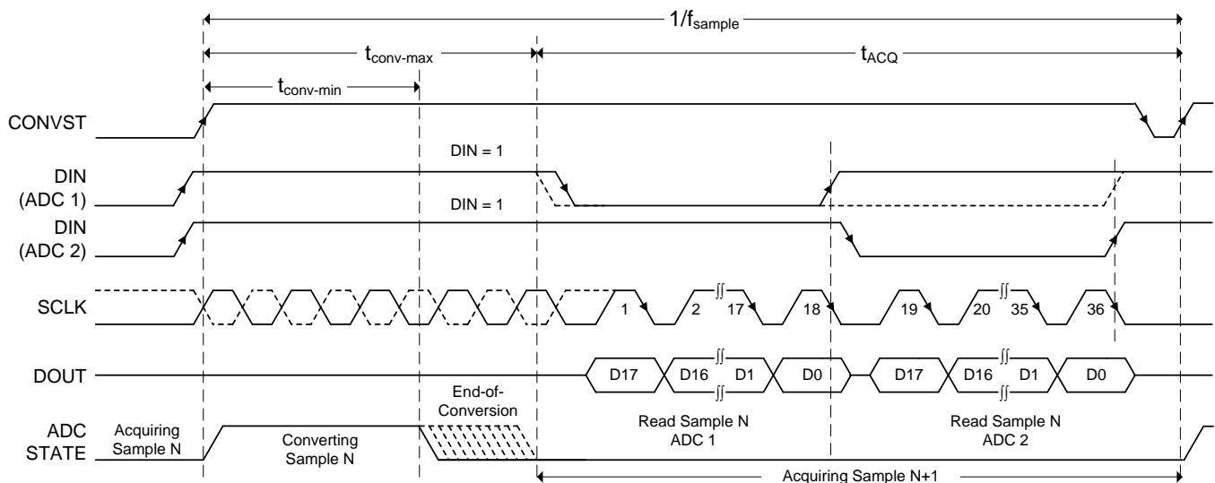
Figure 56. Interface Timing Diagram: Two ADCs with 4-Wire \overline{CS} Mode Without a Busy Indicator
