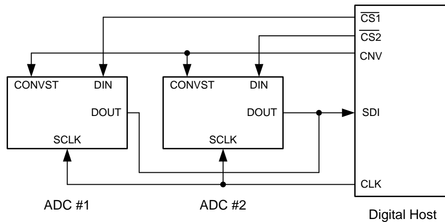
Figure 55. Connection Diagram: Two ADCs with 4-Wire \overline{CS} Mode Without a Busy Indicator
