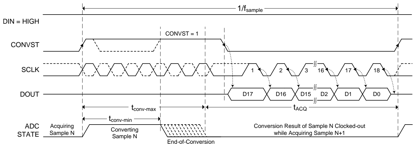
Figure 50. Interface Timing Diagram: 3-Wire \overline{\text{CS}} Mode Without a Busy Indicator (DIN = 1)
