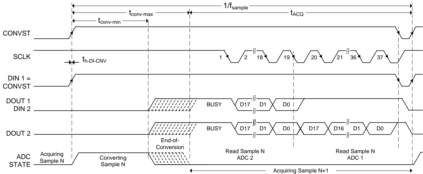
Figure 62. Interface Timing Diagram: For Two Devices in Daisy-Chain Mode With a Busy Indicator
