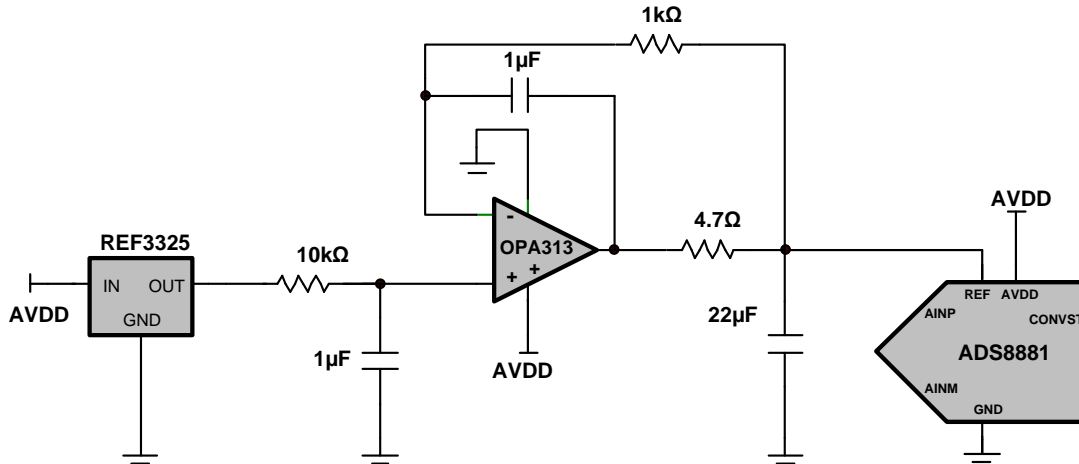
Figure 65. Schematic of Reference Driver Circuit with V_{REF} = 2.5\text{ V DC}
