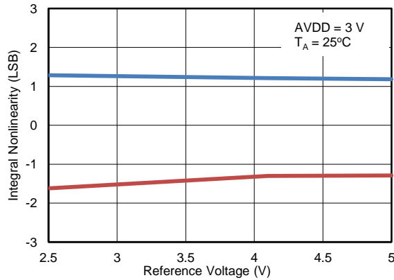
Figure 12. INL vs REFERENCE VOLTAGE
