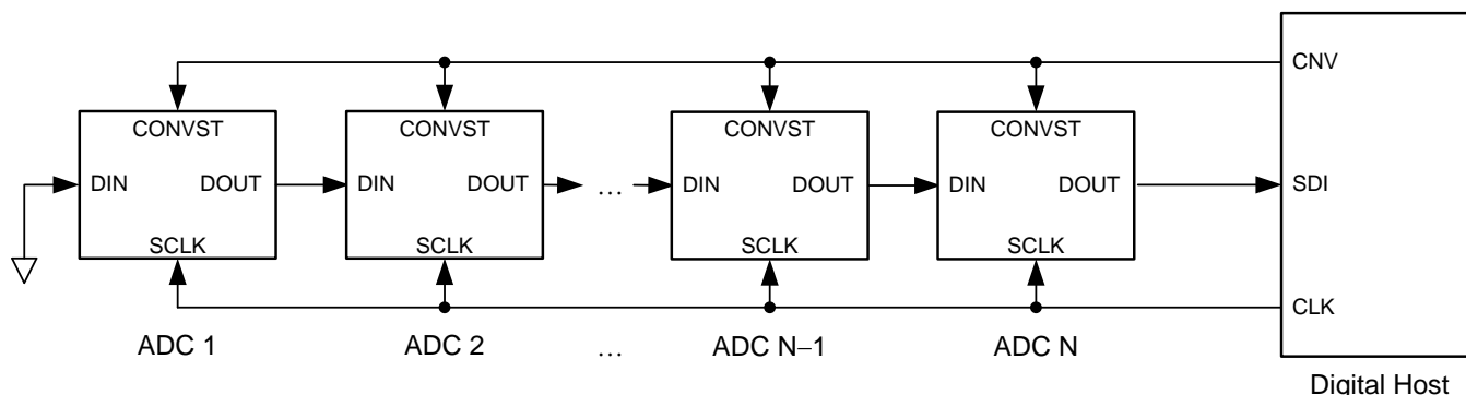
Figure 59. Connection Diagram: Daisy-Chain Mode Without a Busy Indicator ( \text{DIN} = 0 )
