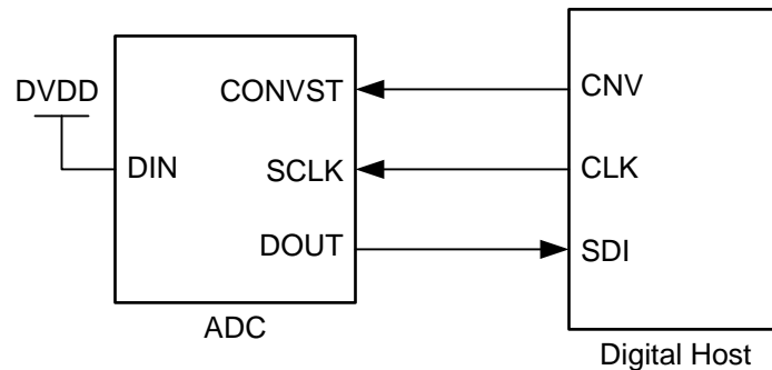
Figure 49. Connection Diagram: 3-Wire \overline{\text{CS}} Mode Without a Busy Indicator (DIN = 1)
