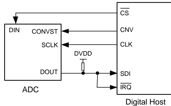
Figure 57. Connection Diagram: 4-Wire \overline{\text{CS}} Mode With a Busy Indicator
