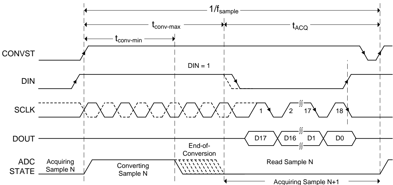
Figure 54. Interface Timing Diagram: Single ADC with 4-Wire \overline{\text{CS}} Mode
