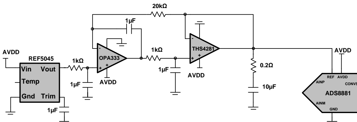
Figure 64. Schematic of Reference Driver Circuit with V_{\text{REF}} = 4.5 \text{ V DC}
