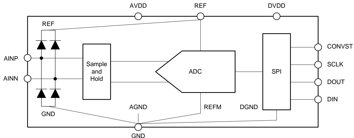
Figure 45. Detailed Block Diagram
