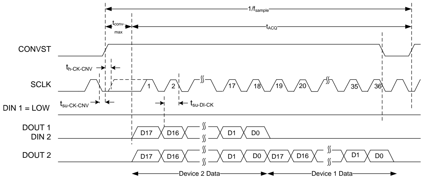
Figure 3. Daisy-Chain Operation - 2 devices
