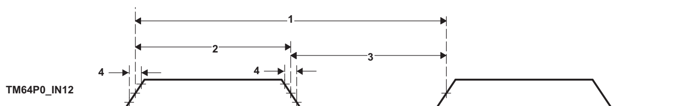
Figure 5-60. Timer Timing
