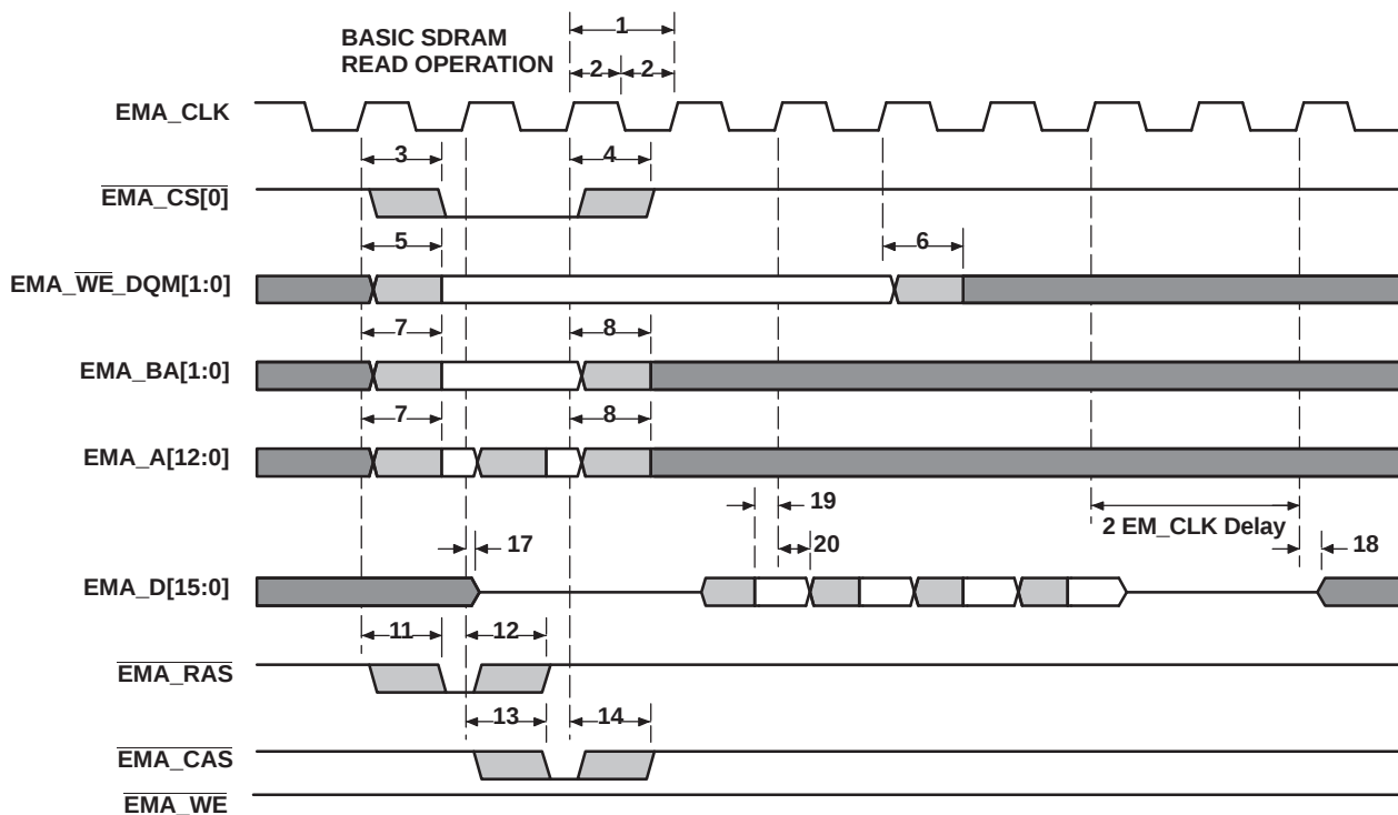
Figure 5-11. EMIFA Basic SDRAM Read Operation
