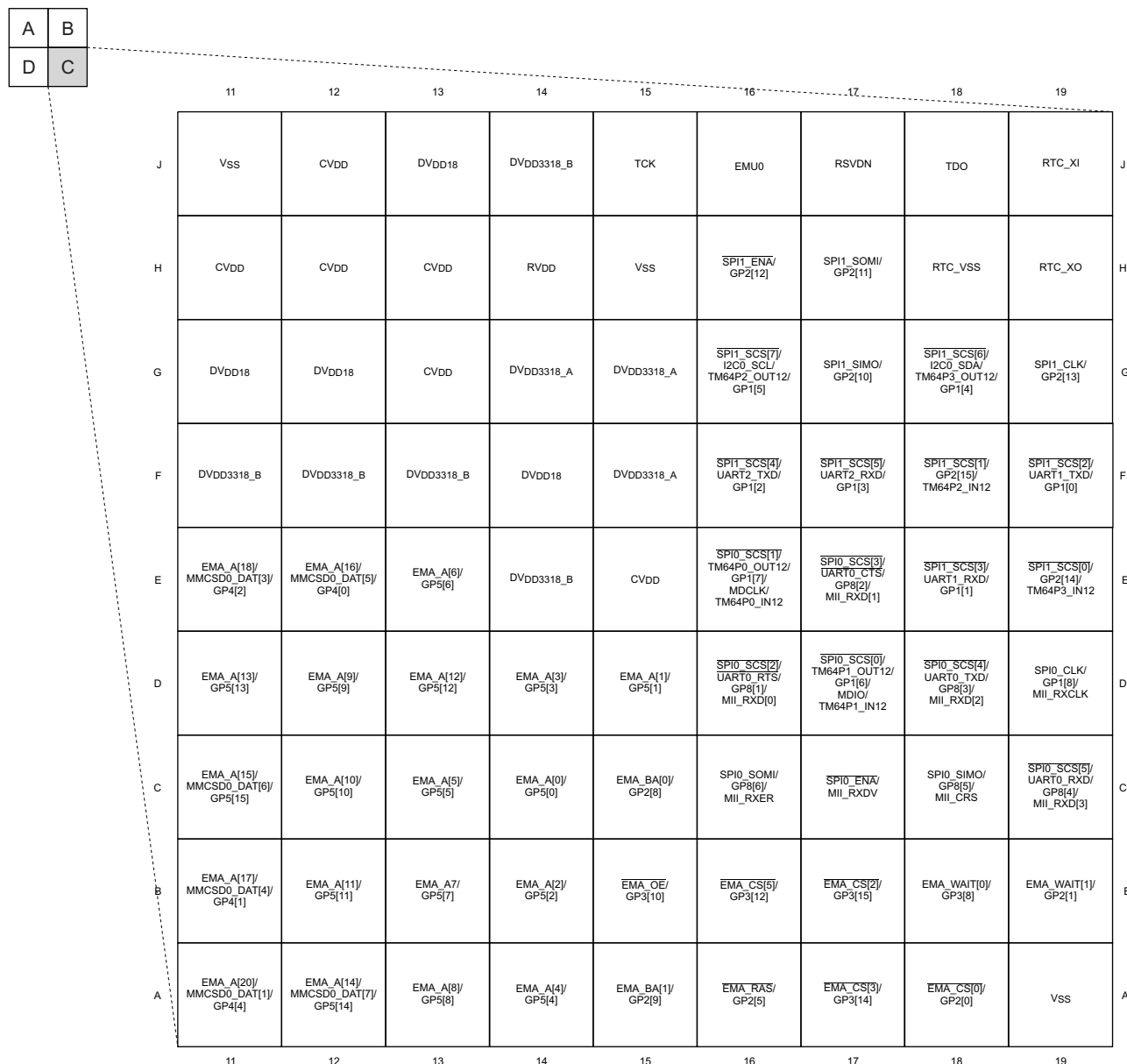
Figure 2-3. Pin Map (Quad C)
