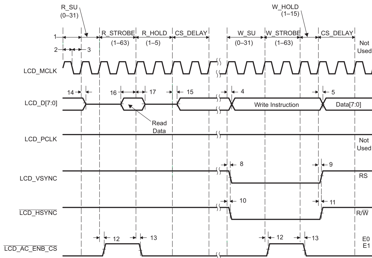
Figure 5-53. Character Display HD44780 Read
