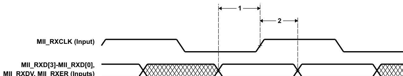
Figure 5-47. EMAC Receive Interface Timing
