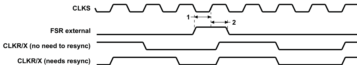
Figure 5-33. FSR Timing When GSYNC = 1
