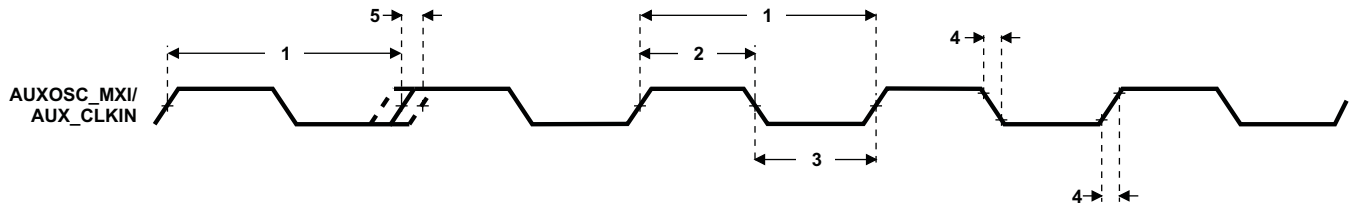
Figure 7-13. AUX_MXI/AUX_CLKIN Timing
