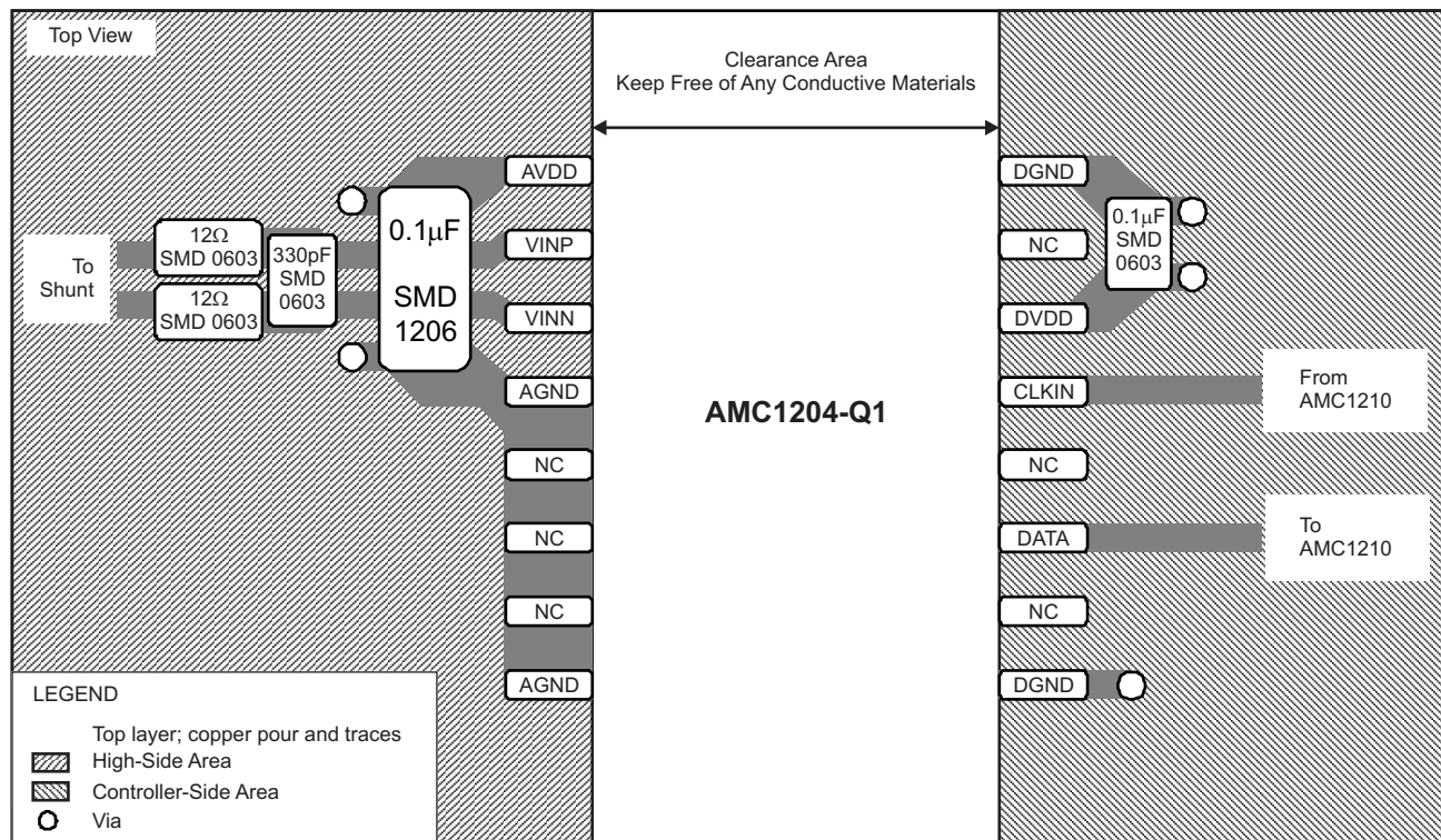
Figure 52. Recommended Layout
