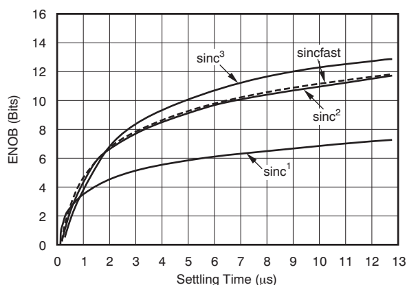
Figure 49. Measured Effective Number of Bits versus Settling Time
