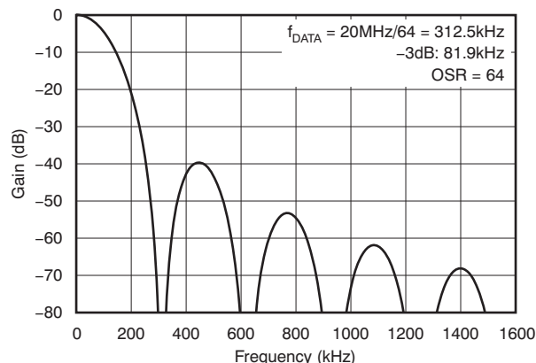
Figure 46. Frequency Response of the \text{Sinc}^3 Filter
