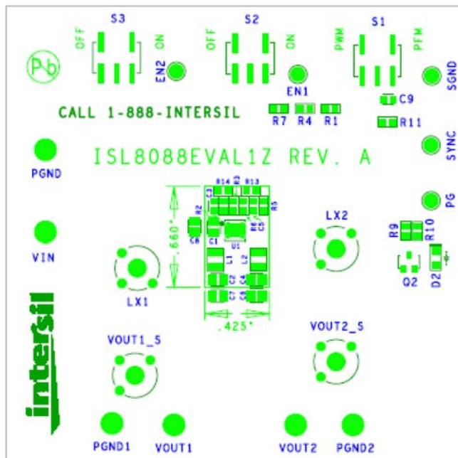
FIGURE 1. TOP COMPONENTS
