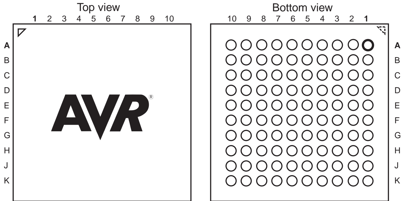
Figure 2-2. BGA-pinout
