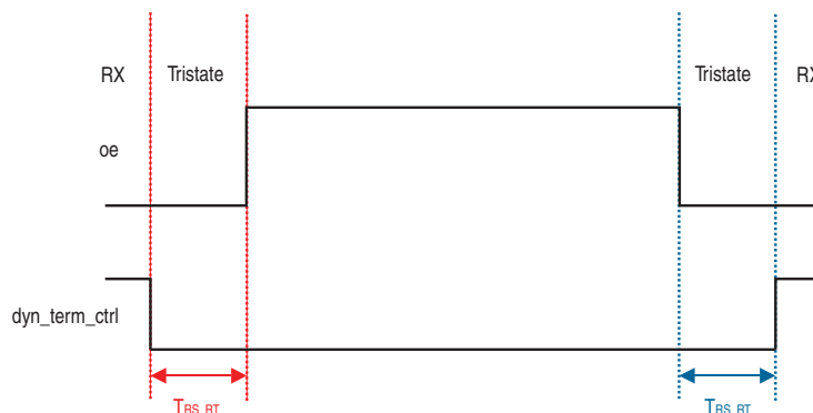
Figure 2–4. Timing Diagram for dyn_term_ctrl and oe Signals
