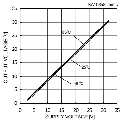
Fig. 4 Maximum Output Voltage - Supply Voltage ( R_L=10[k\Omega] )
