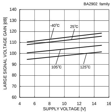
Large Signal Voltage Gain - Supply Voltage ( R_L=2[k\Omega] )
