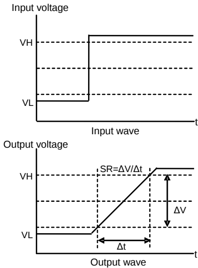
Fig. 123 Slew Rate Input Waveform
