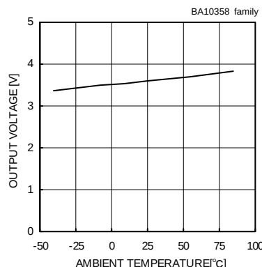
Fig. 5 Maximum Output Voltage - Ambient Temperature ( V_{CC}=5[V] , R_L=2[k\Omega] )
