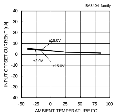
Fig. 108 Input Offset Current - Ambient Temperature (Vicm=0[V], VOUT=0[V])
