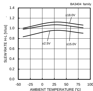
Fig. 116 Slew Rate H-L - Ambient Temperature
