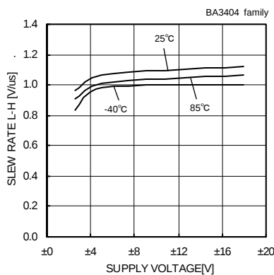
Fig. 115 Slew Rate L-H - Supply Voltage
