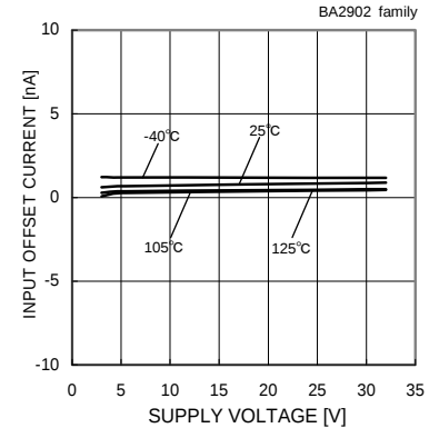
Input Offset Current - Supply Voltage ( V_{icm}=0[V] , V_{OUT}=1.4[V] )
