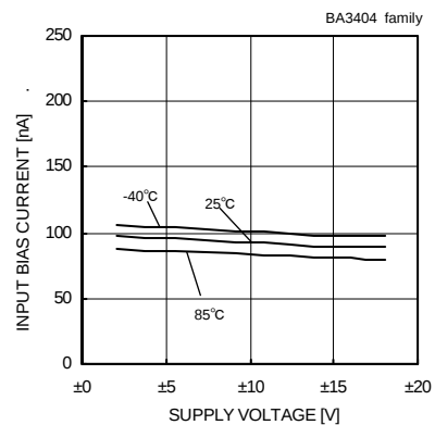
Fig. 105 Input Bias Current - Supply Voltage (Vicm=0[V], VOUT=0[V])
