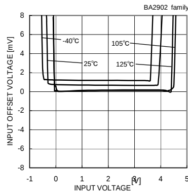
Input Offset Voltage - Common Mode Input Voltage ( V_{CC}=5[V] )
