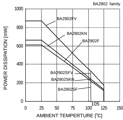
Derating Curve
