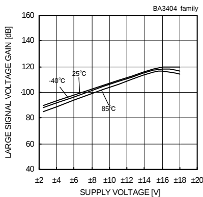
Fig. 112 Large Signal Voltage Gain - Supply Voltage (RL=2[kΩ])
