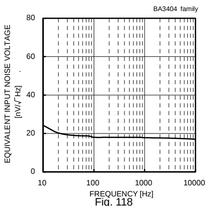
Fig. 118 Equivalent Input Noise Voltage - Frequency (VCC/VEE=+15[V]/-15[V], Rs=100[Ω], Ta=25[°C])
