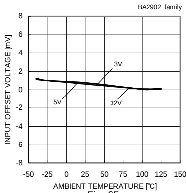
Input Offset Voltage - Ambient Temperature ( V_{icm}=0[V] , V_{OUT}=1.4[V] )
