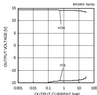
Fig. 102 Output Voltage - Output Current (VCC/VEE=+15[V]/-15[V], Ta=25[°C])
