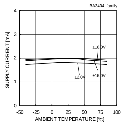
Fig. 99 Supply Current - Ambient Temperature
