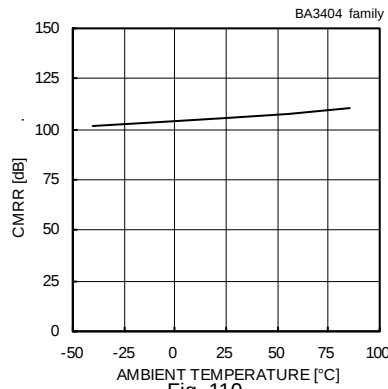
Fig. 110 Common Mode Rejection Ratio - Ambient Temperature (VCC/VEE=+15[V]/-15[V])
