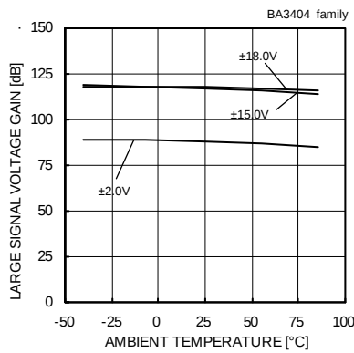
Fig. 113 Large Signal Voltage Gain - Ambient Temperature (RL=2[kΩ])
