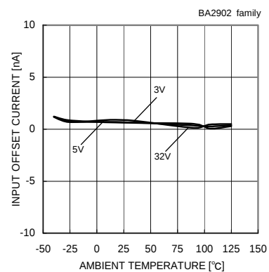
Input Offset Current - Ambient Temperature ( V_{icm}=0[V] , V_{OUT}=1.4[V] )
