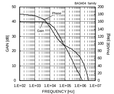
Fig. 114 Voltage Gain - Frequency (VCC=±15V)
