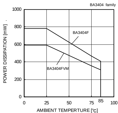
Fig. 97 Derating Curve
