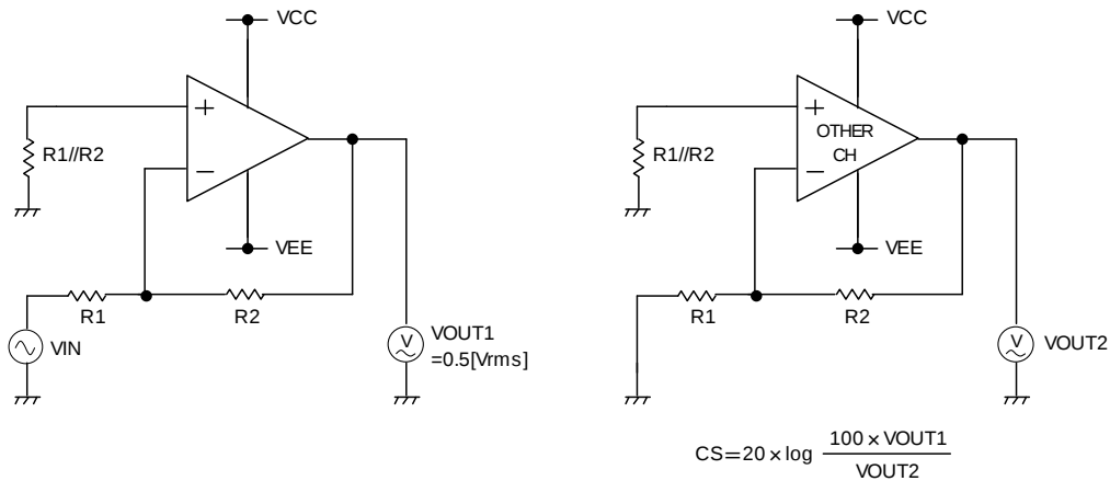
Fig. 124 Test Circuit 3
