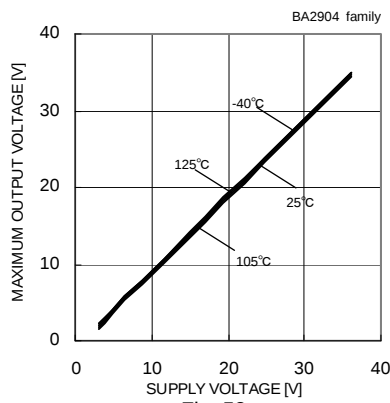
Fig. 52 Maximum Output Voltage - Supply Voltage ( R_L=10[k\Omega] )
