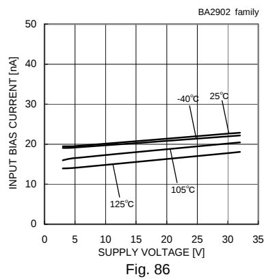
Input Bias Current - Supply Voltage ( V_{icm}=0[V] , V_{OUT}=1.4[V] )
