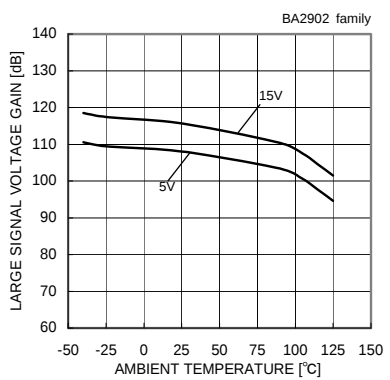
Large Signal Voltage Gain - Ambient Temperature ( R_L=2[k\Omega] )
