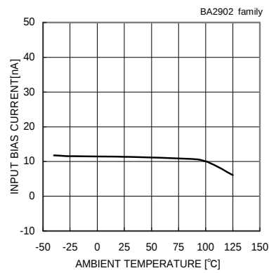
Input Bias Current - Ambient Temperature ( V_{CC}=30[V] , V_{icm}=28[V] , V_{OUT}=1.4[V] )
