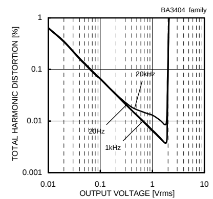
Fig. 117 Total Harmonic Distortion - Output Voltage (VCC/VEE=+4[V]/-4[V], Av=0[dB], RL=2[kΩ], 80[kHz]-LPF, Ta=25[°C])
