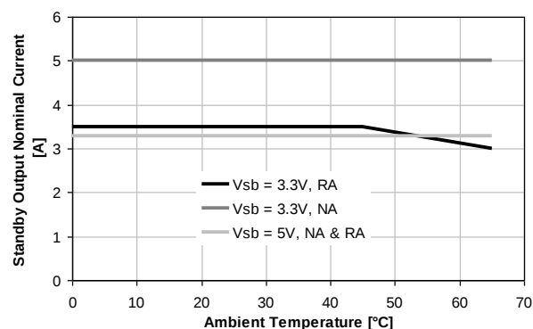
Figure 23 - Temperature derating on V_{SB}
