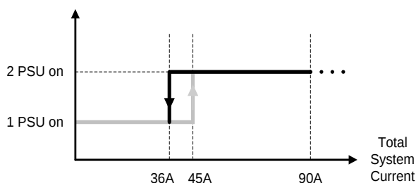
Figure 32 - Recommended hot-standby configuration
