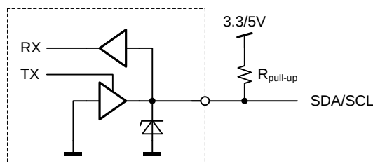
Figure 33 - Physical layer of communication interface
