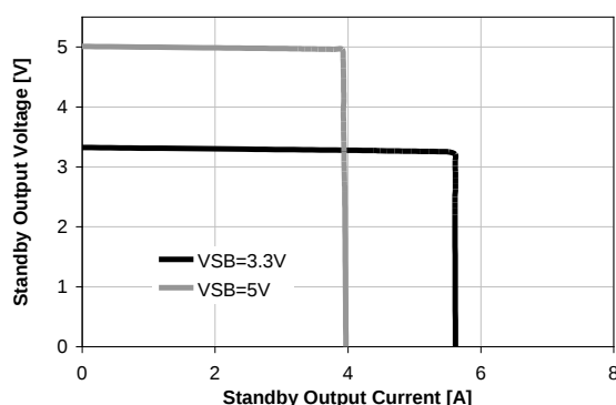
Figure 22 - Current limitation on V_{SB}
