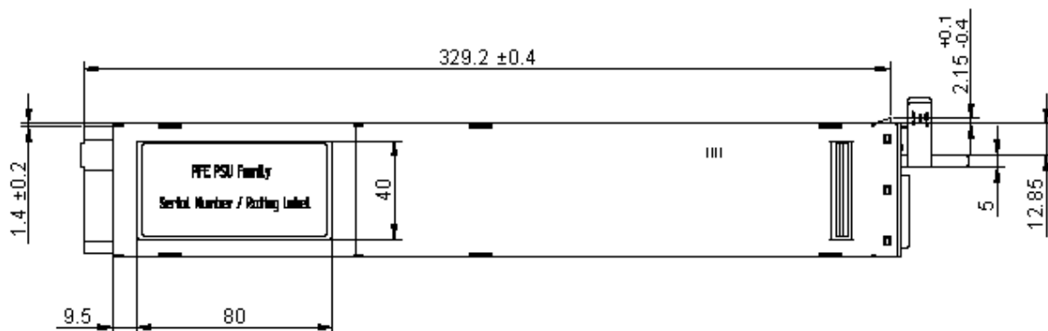
Figure 45 - Side View 2
