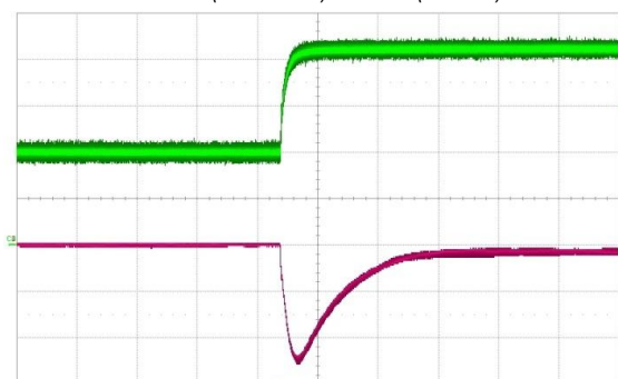
Figure 177 - Load transient V_1 , 40 to 85A (500 \mu s/div) CH2: V_1 (200mV/div) CH4: I_1 (20A/div)
