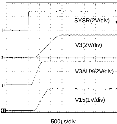
Fig.7 Wakeup Wave Form (Standby→Active)
