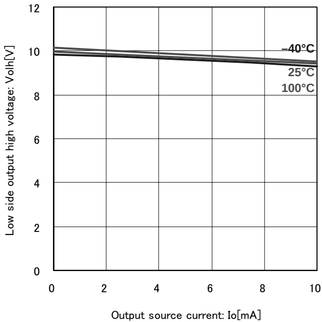
Fig.7 Low side output high voltage (Vcc=12V)
