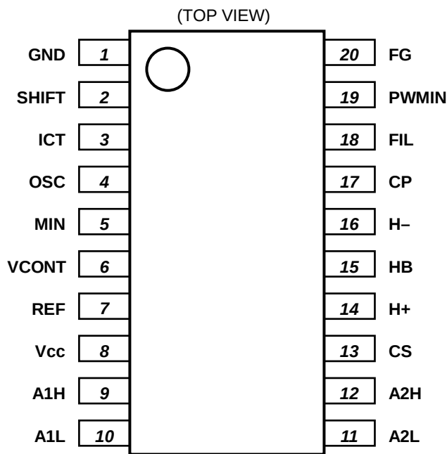
Fig.1 Pin configuration
