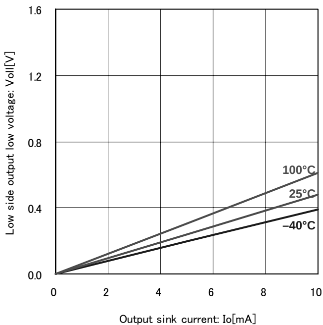
Fig.9 Low side output low voltage (Vcc=12V)
