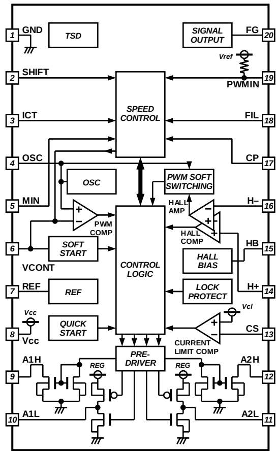
Fig.2 Block diagram
