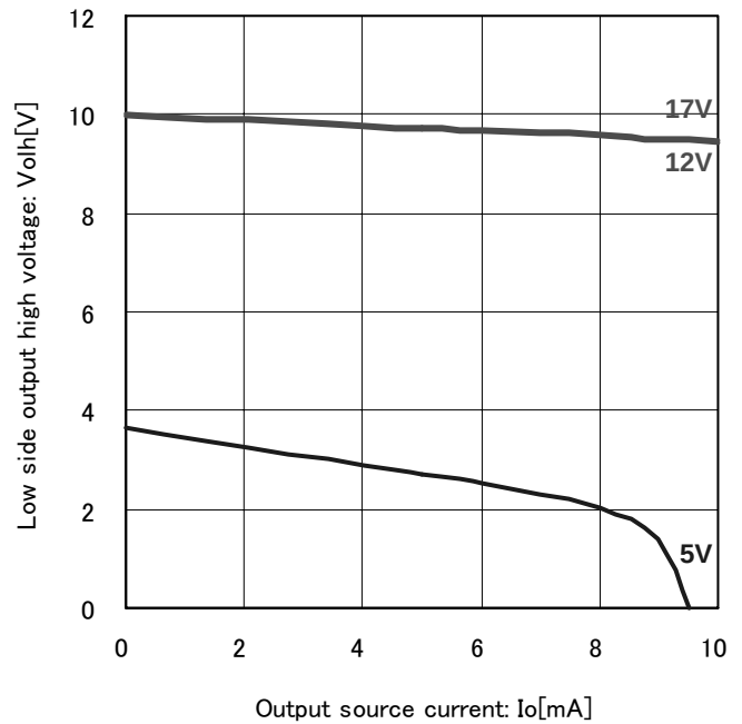
Fig.8 Low side output high voltage (Ta=25°C)
