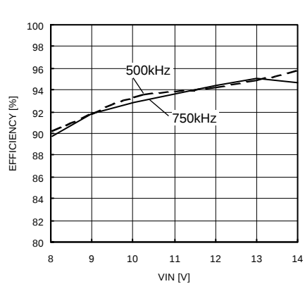
Fig.18 STEP UP EFFICIENCY
