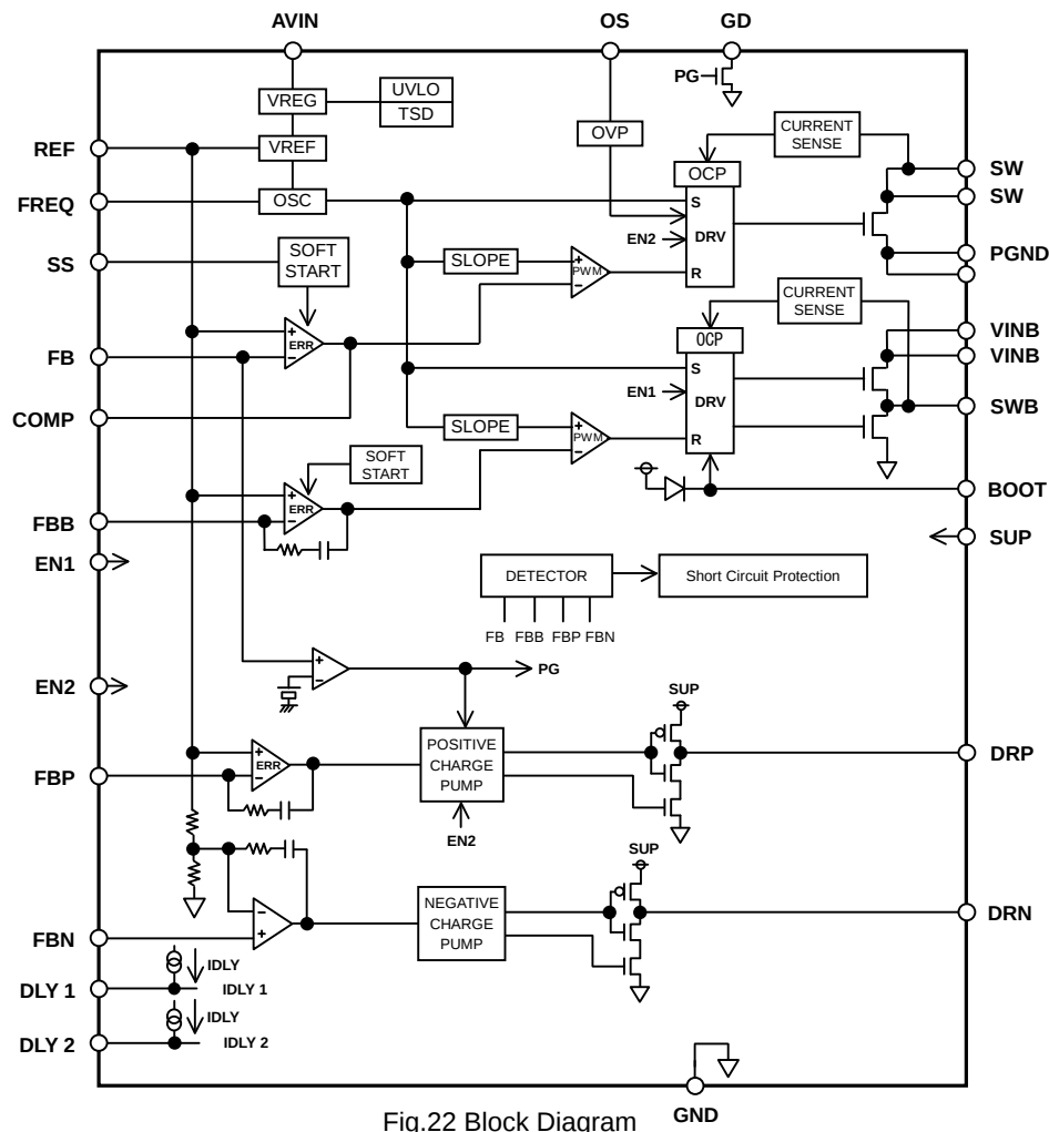
Fig.22 Block Diagram
