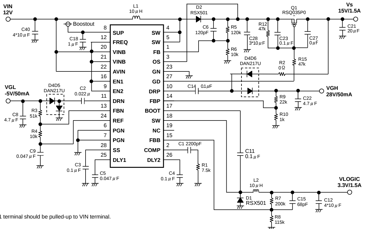
Fig.23 Typical Application
