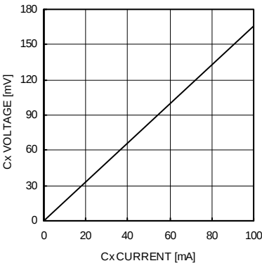
Fig.24 Charge Pump P-channel On Resistance
