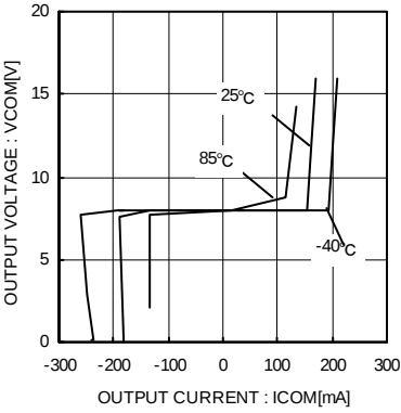
Fig.15 COM Load Regulation
