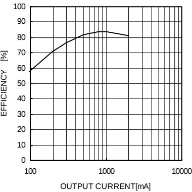
Fig.20 Output Current vs Efficiency (VDD)
