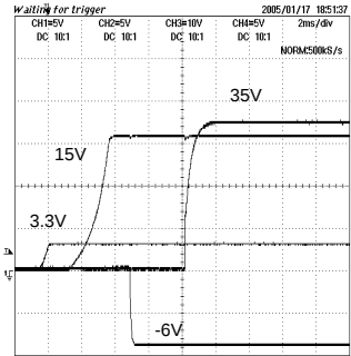
Fig.17 Start-up Sequence
