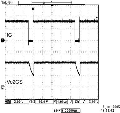
Fig.18 Gate-shading Waveform
