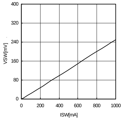
Fig.22 DC/DC SW On Resistance
