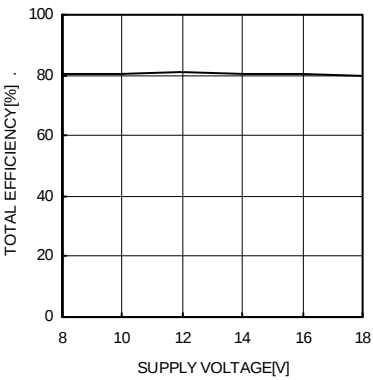
Fig.21 Total Efficiency
