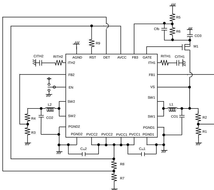
Fig.40 Typical application
