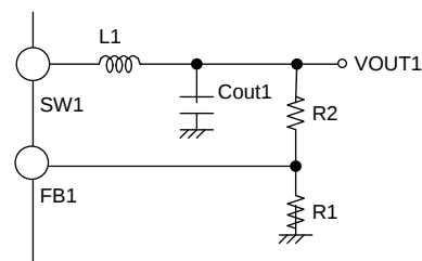
Fig.41 Determination of output voltage
