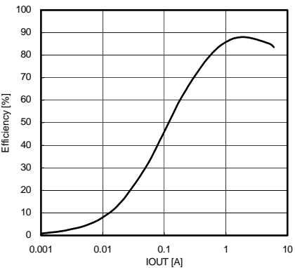
Fig.23 efficiency (2ch)
