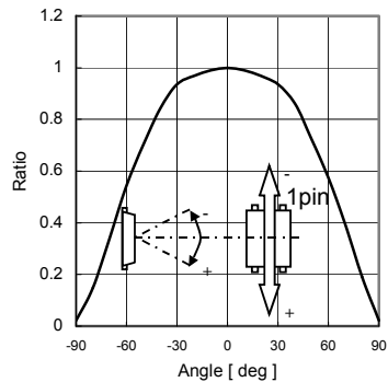
Fig.5 Directional Characteristics 2
