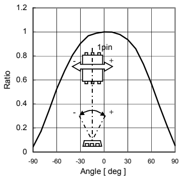
Fig.4 Directional Characteristics 1
