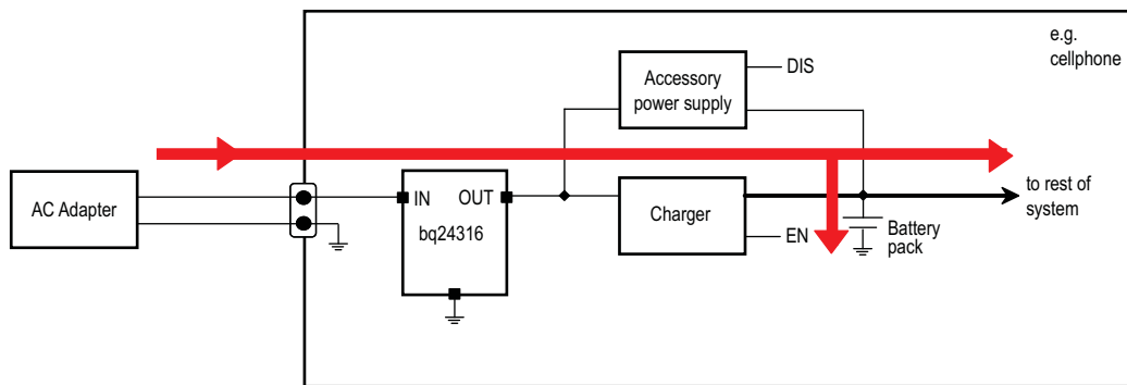
Figure 25. Charging - The Red Arrows Show the Direction of Current Flow
