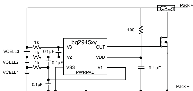
Figure 8. 3-Series Cell Configuration with Fixed Delay
