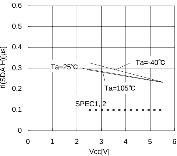
Figure 29. Noise removal valid time tI(SDA H)
