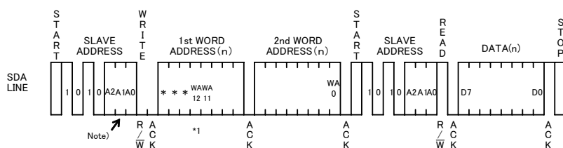
Figure 42. Random read cycle (BR24A32/64 -WM)
