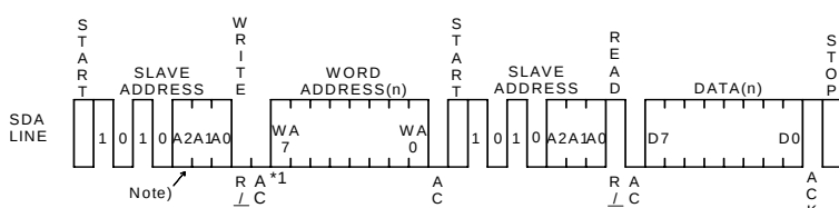
Figure 41. Random read cycle (BR24A01A/02/04/08/16-WM)
