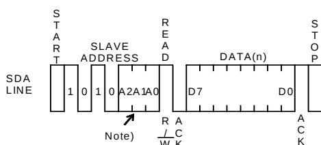
Figure 43. Current read cycle
