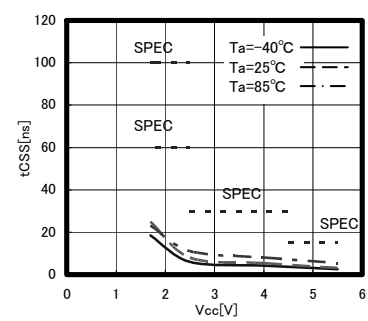
Fig.20 CSB setup time t_{CSS}
