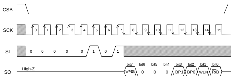
Fig.38 Read status register command
