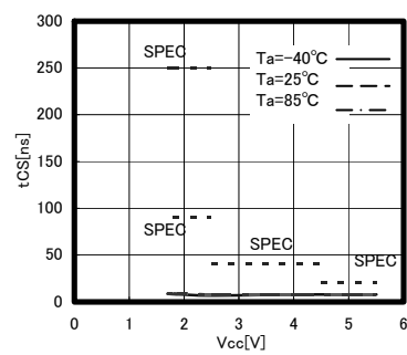
Fig.19 CSB high time t_{CS}
