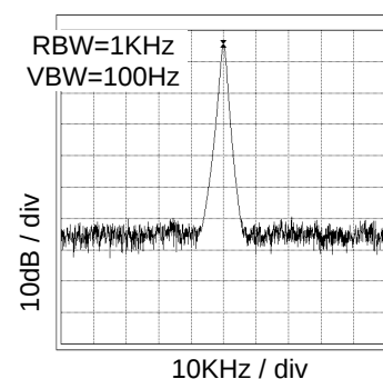
Fig.6 27MHz Spectrum VDD=3.3V at CL=15pF
