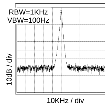
Fig.9 13.5MHz Spectrum VDD=3.3V, at CL=15pF
