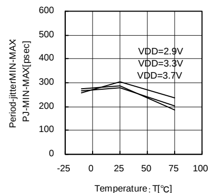
Fig.39 36.9MHz Temperature—Period-Jitter MIN-MAX
