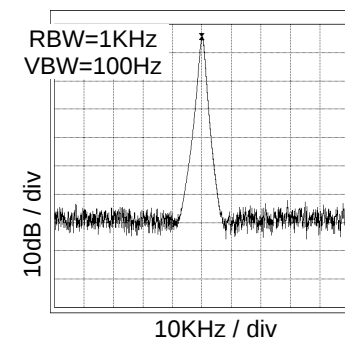
Fig.12 33.9MHz Spectrum VDD=3.3V, at CL=15pF
