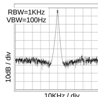
Fig.52 33.9MHz Spectrum VDD=3.3V, at CL=15pF
