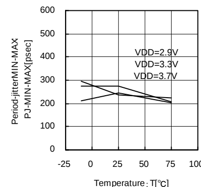
Fig.42 18.4MHz Temperature—Period-Jitter MIN-MAX
