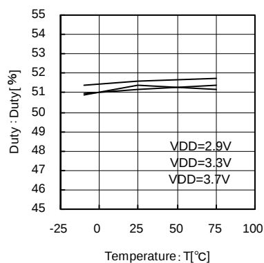
Fig.40 18.4MHz Temperature—Duty
