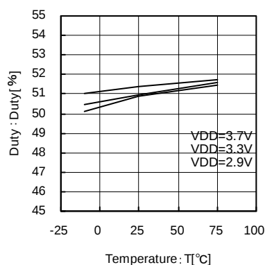
Fig.37 36.9MHz Temperature—Duty
