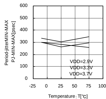
Fig.36 16.9MHz Temperature—Period-Jitter MIN-MAX
